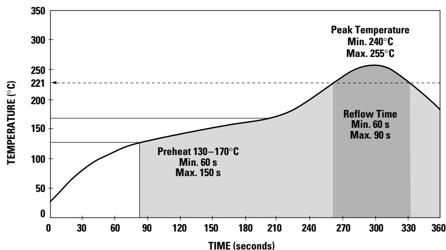
Figure 23. Surface Mount Assembly Temperature Profile.
