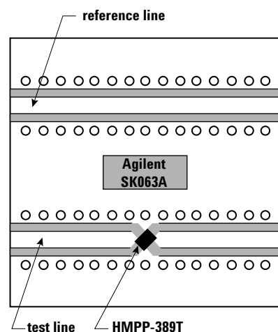
Figure 12. Demo-board DEMO-HMPP-389T.
