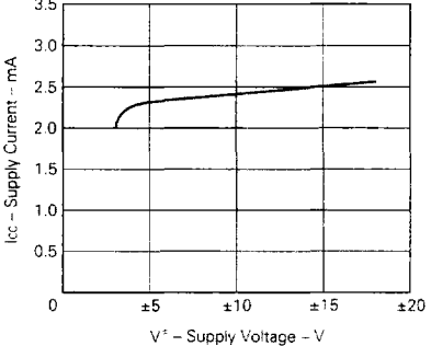
SUPPLY CURRENT
