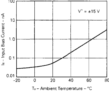
INPUT BIAS CURRENT
