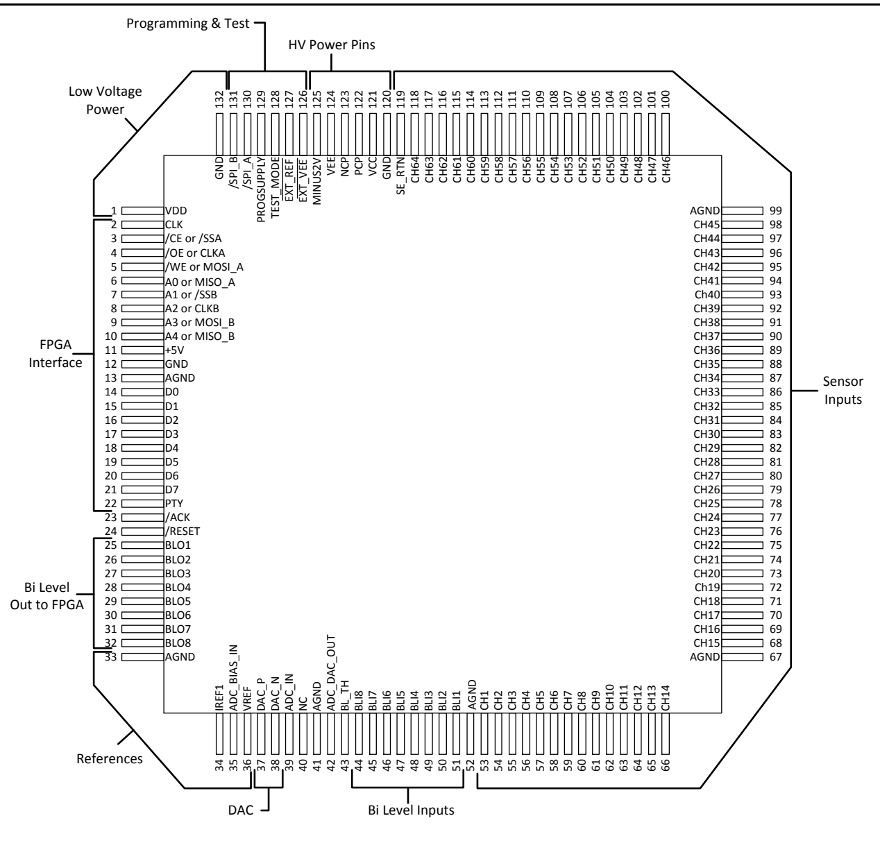
Figure 2 · Pinout
