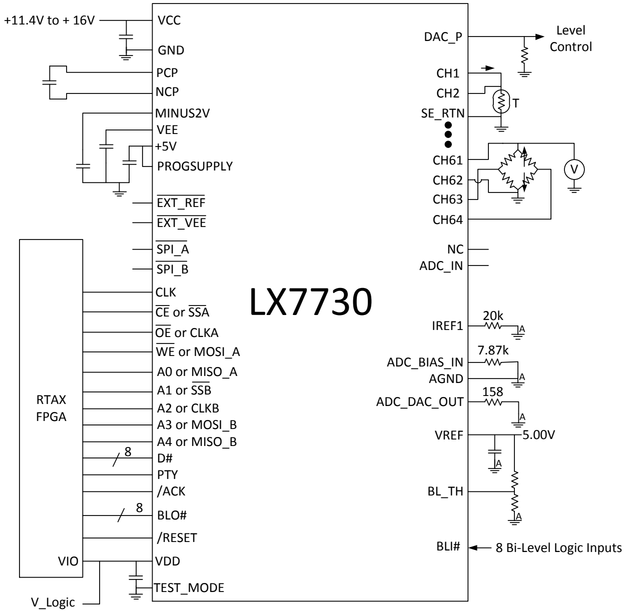
Figure 5 · Typical Application
