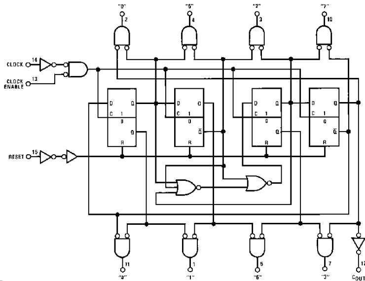
CD4022B
