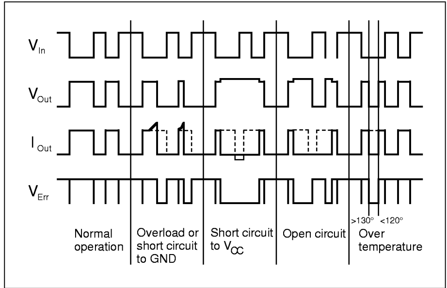
Figure 18. Signal diagram
