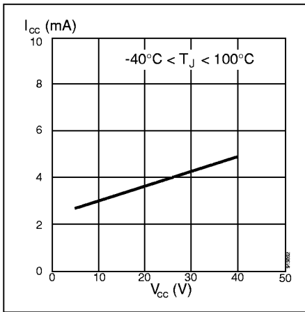
Figure 7. Current consumption vs. supply voltage at 2\text{ V} \leq V_{in} \leq V_{cc} V. (Inactive output)
