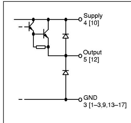
Figure 16. Output stage.
