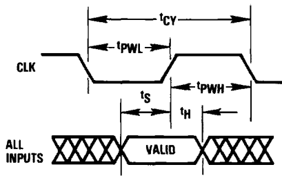
Figure 3. Input/Clock Timing
