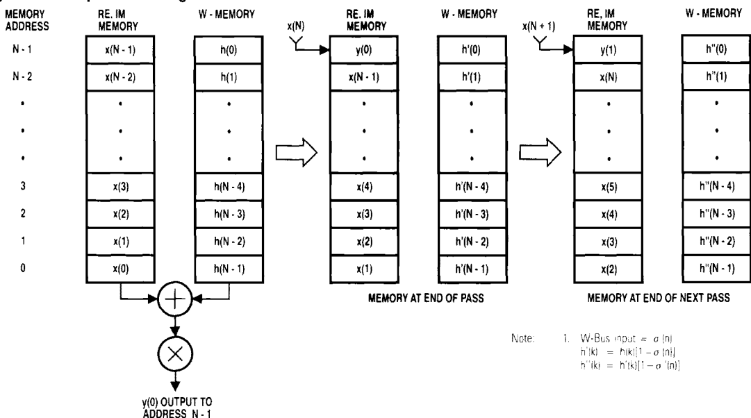
Figure 18. Adaptive Filtering
