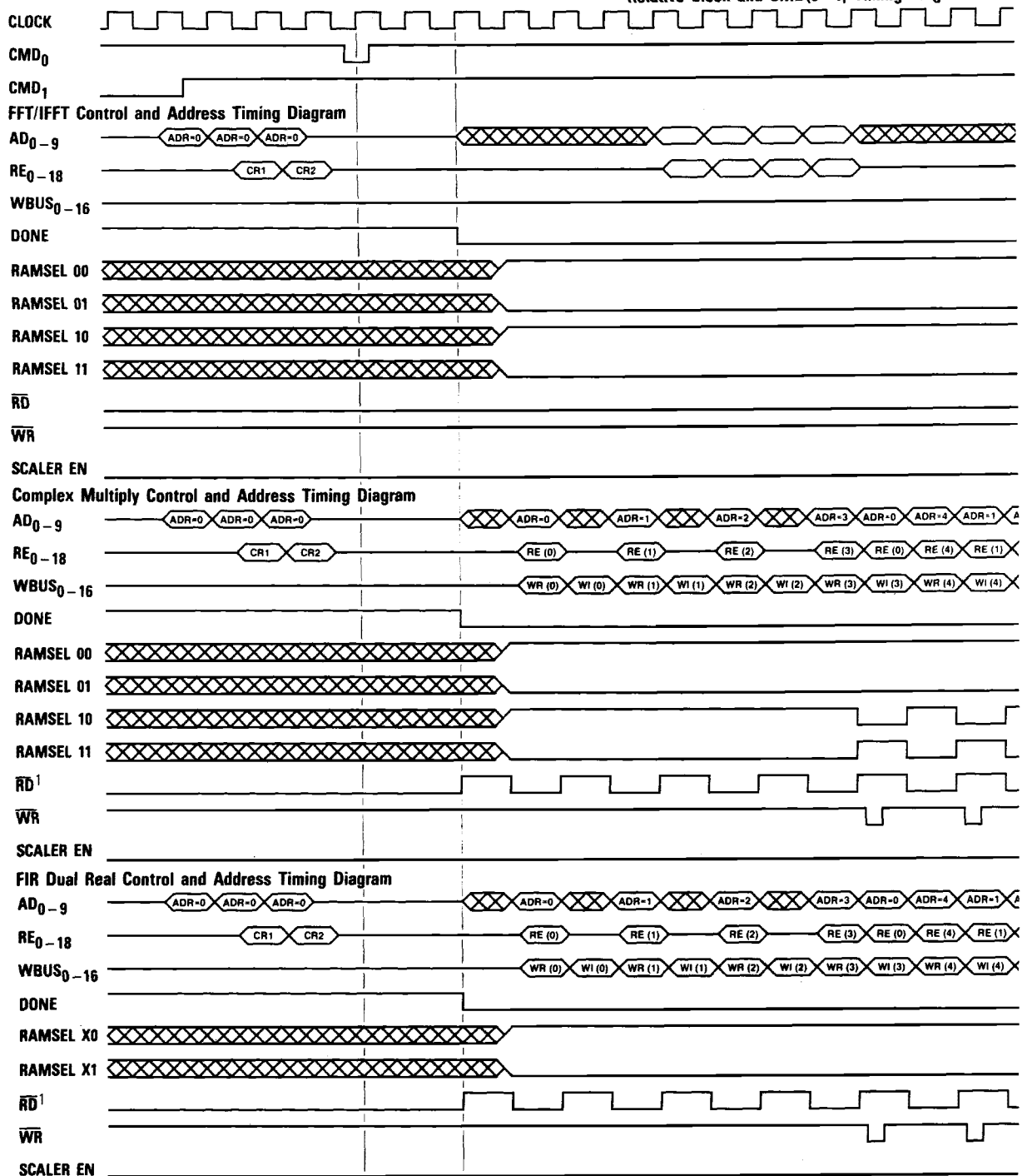
Figure 11. TMC2310 Overall Timing Diagram – Normal Addressing Relative Clock and CMD(0–1) Timing Diagram
