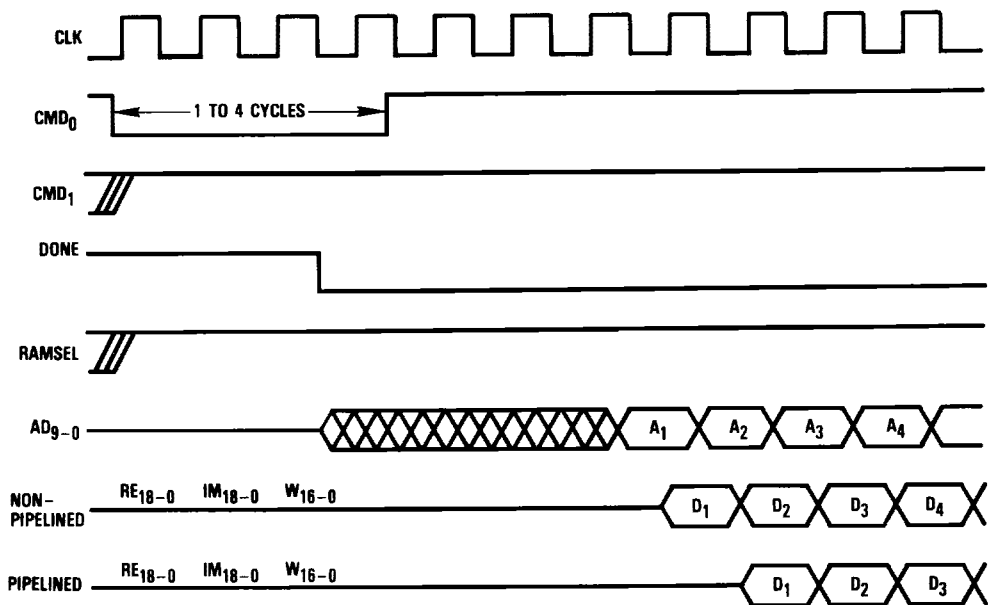
Figure 9. START Timing (Shown for FFT/IFFT with Windowing)
