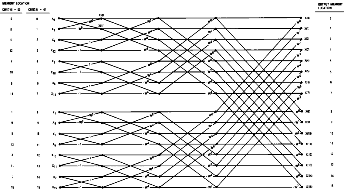
Figure 21. 16-Point FFT
