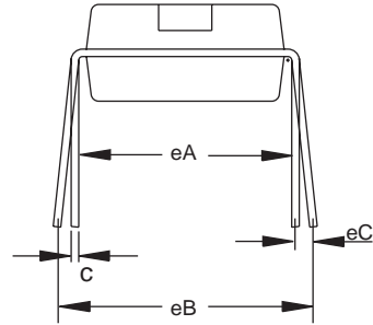
End View
