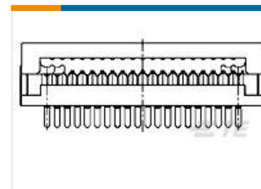
TE Model / Part #2-6437006-3 609-3443LF = PCB IDC P 34 ST .125
