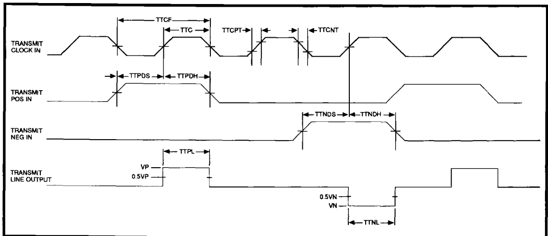
FIGURE 3: Transmit Waveforms
