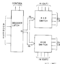
CD22101, CD22102 Functional Diagram
