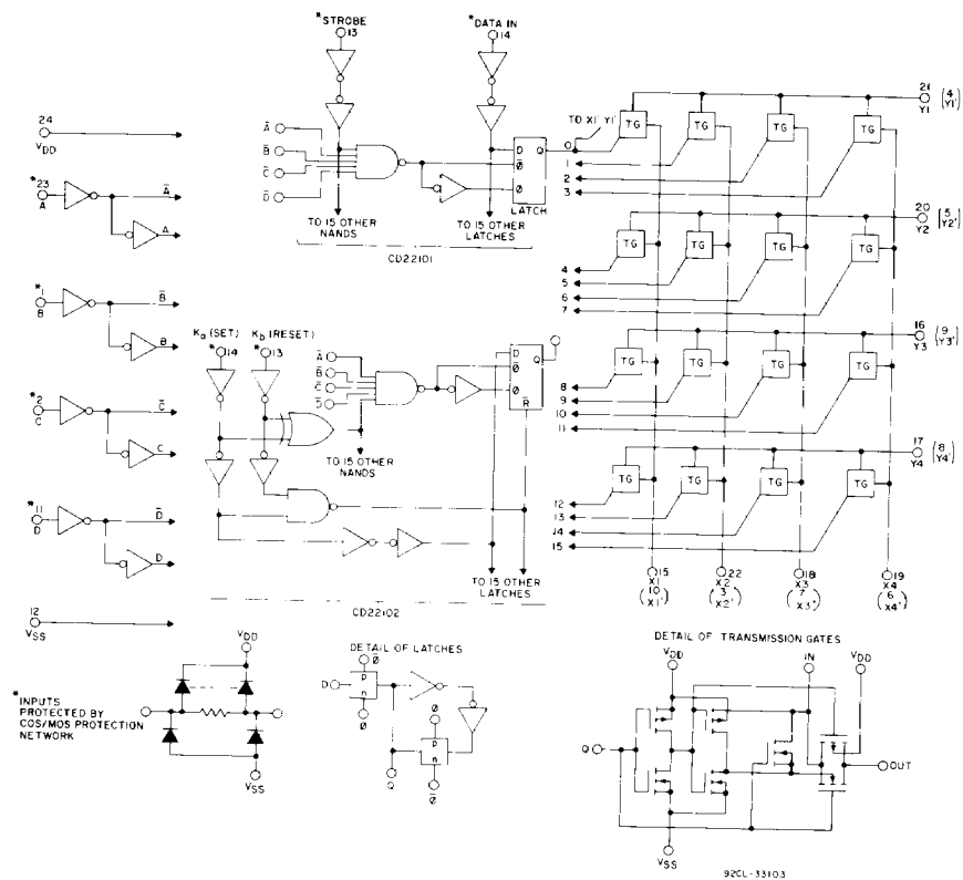
Fig. 2 — Logic diagram.
