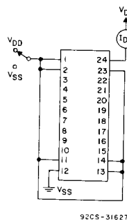
Fig. 12 - Quiescent current test circuit.
