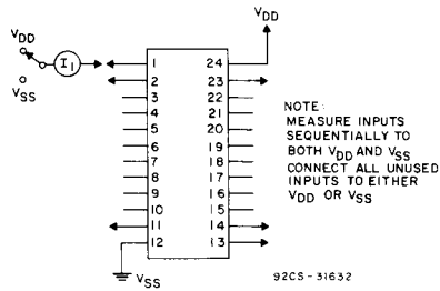
Fig. 13 - Input current test circuit.
