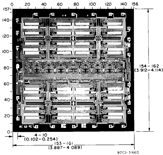
Dimensions and pad layout for CD22102H.
