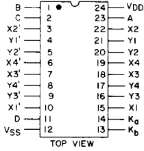
92CS-29840 CD22102 Terminal Diagram
