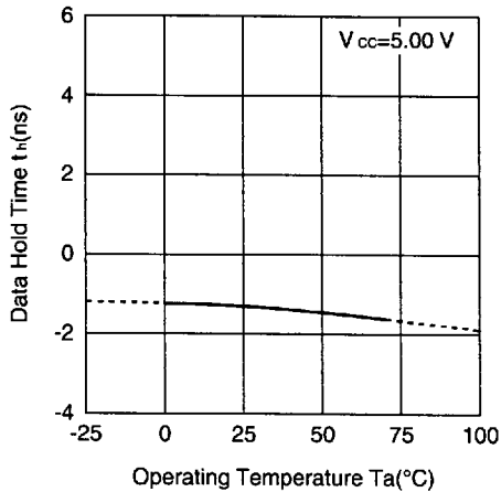
Figure 17 Data Hold Time vs. Operating Temperature
