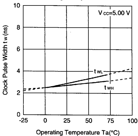
Figure 23 Clock Pulse Width vs. Operating Temperature
