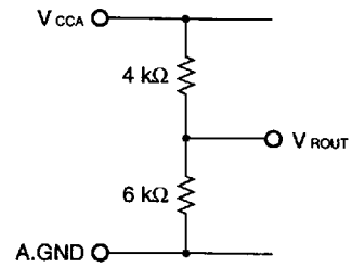
Figure 6 MB40968V Reference Output Voltage (V ROUT )
