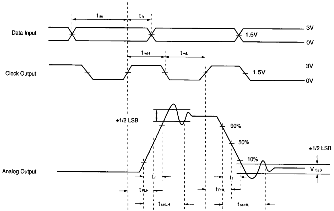
Figure 2 Timing Diagram
