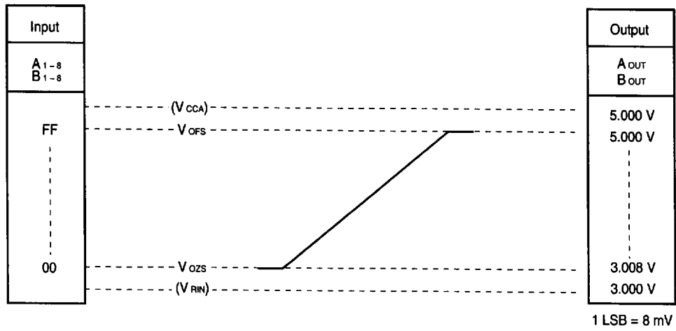
Figure 1 DAC Output Voltage
