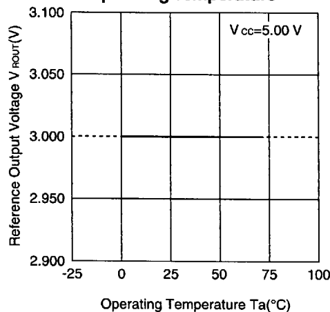
Figure 12 MB40968 Reference Output Voltage vs. Operating Temperature
