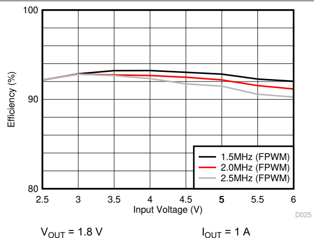
Figure 9-26. Efficiency with Different Switching Frequency
