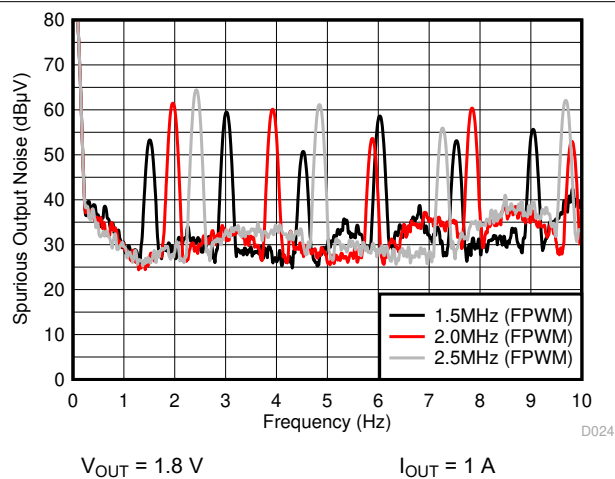
Figure 9-25. Spurious Output Noise with Different Switching Frequency
