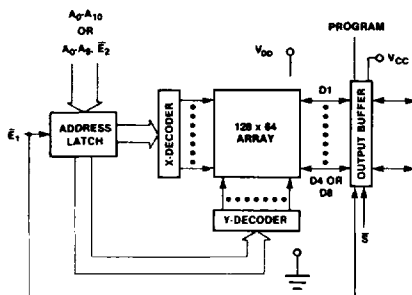
Figure 1: Functional Diagram
