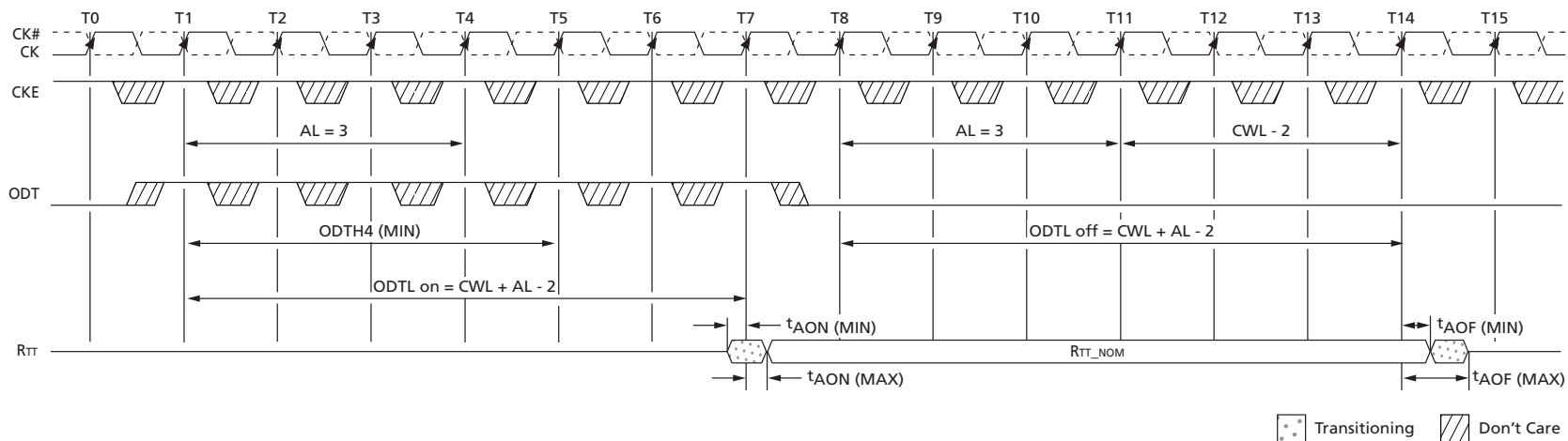
Figure 113: Synchronous ODT
