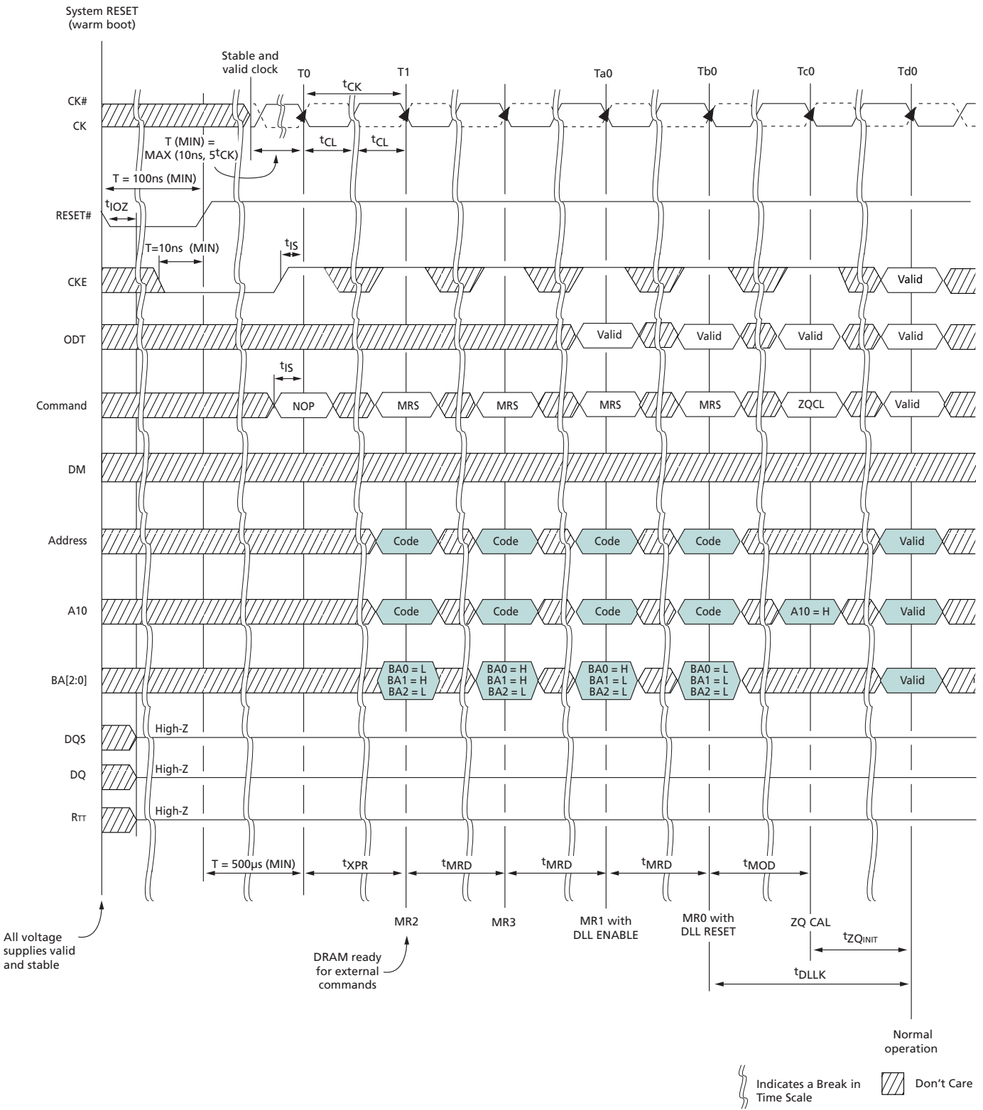
Figure 106: RESET Sequence
