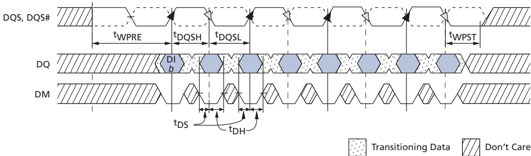
Figure 93: Data Input Timing
