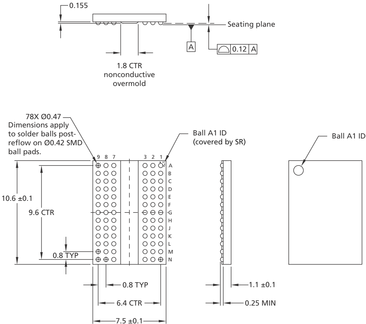
Figure 9: 78-Ball FBGA – x4, x8; “RGF”
