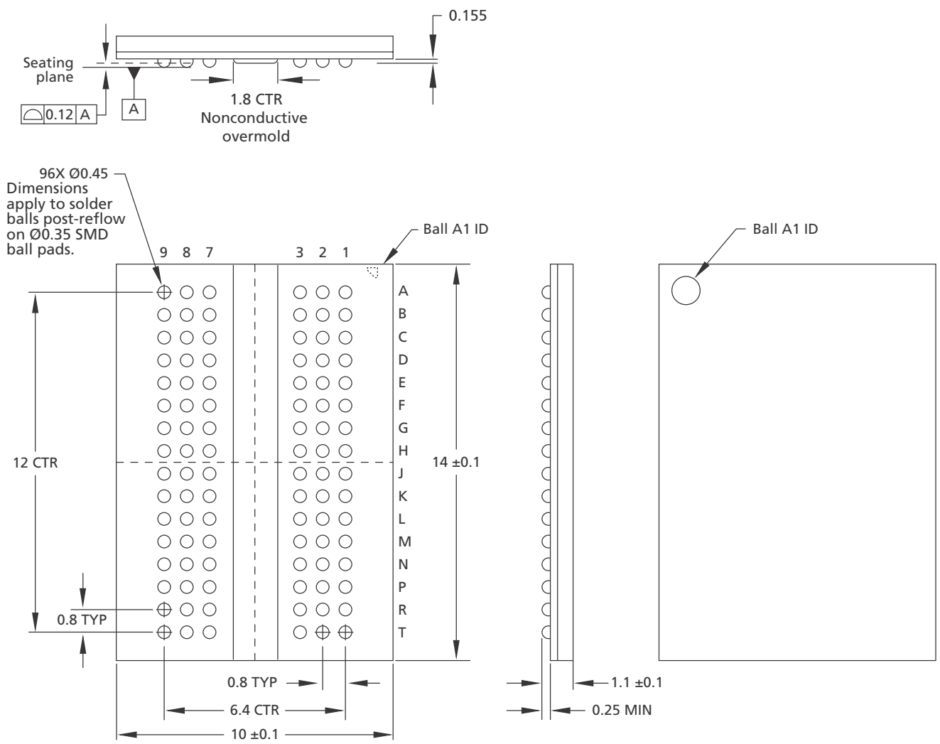
Figure 10: 96-Ball FBGA – x16; “REF”
