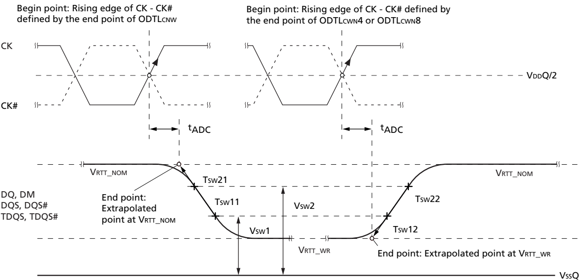
Figure 25: t_{ADC} Definition
