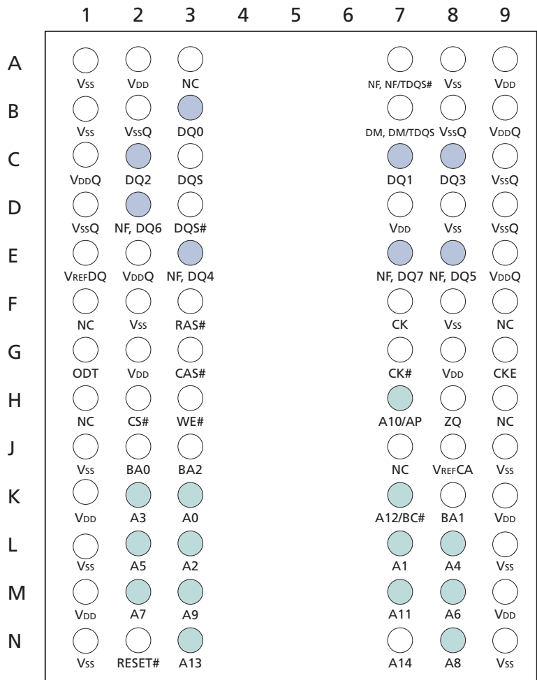
Figure 5: 78-Ball FBGA – x4, x8 Ball Assignments (Top View)
