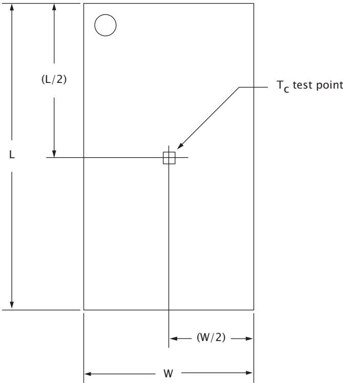
Figure 12: Thermal Measurement Point
