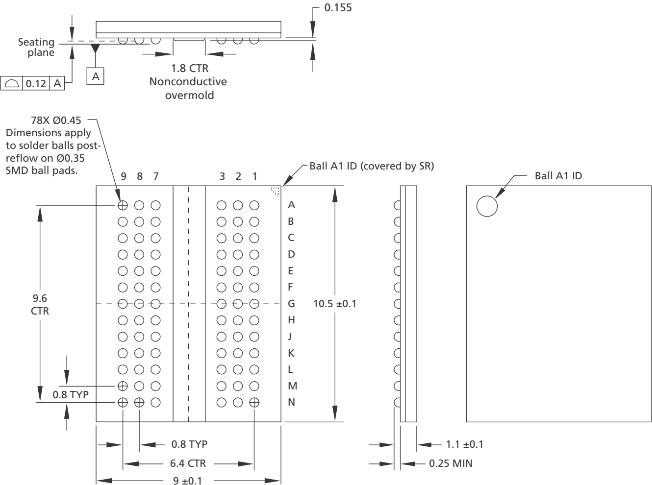
Figure 8: 78-Ball FBGA – x4, x8; “RHF”
