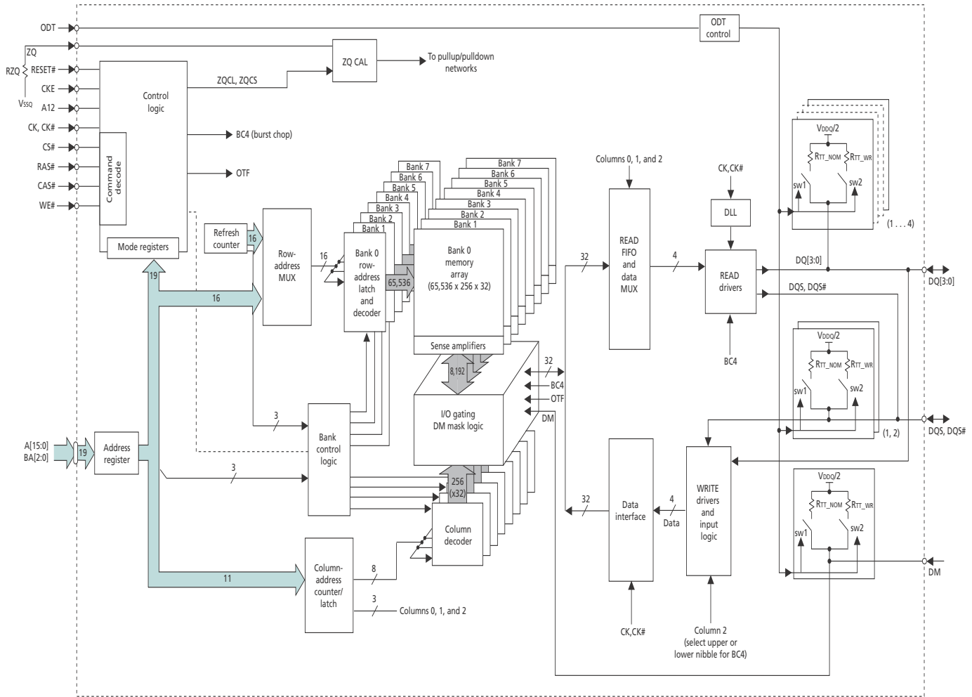
Figure 2: 1 Gig x 4 Functional Block Diagram
