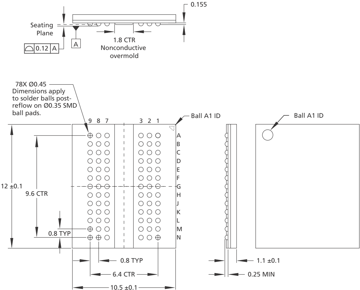
Figure 7: 78-Ball FBGA – x4, x8; “RAF”
