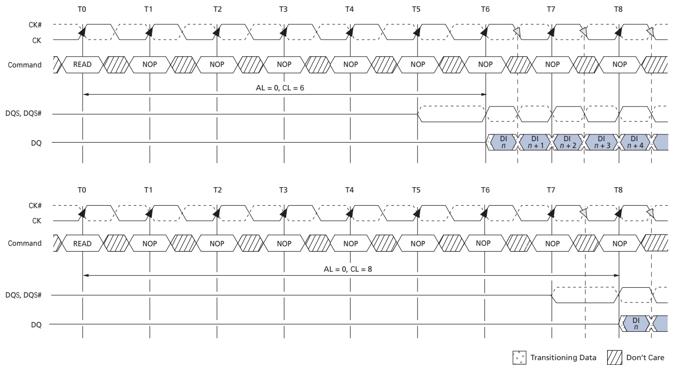
Figure 52: READ Latency
