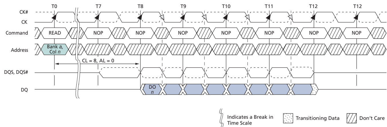
Figure 66: READ Latency
