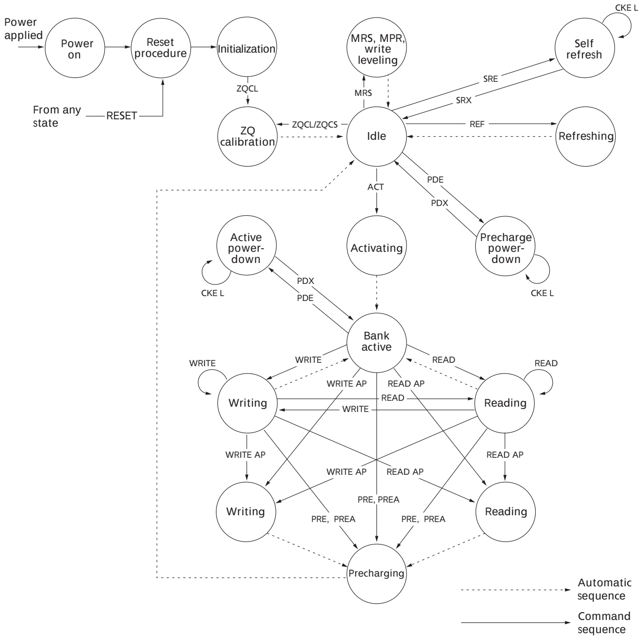
Figure 1: Simplified State Diagram
