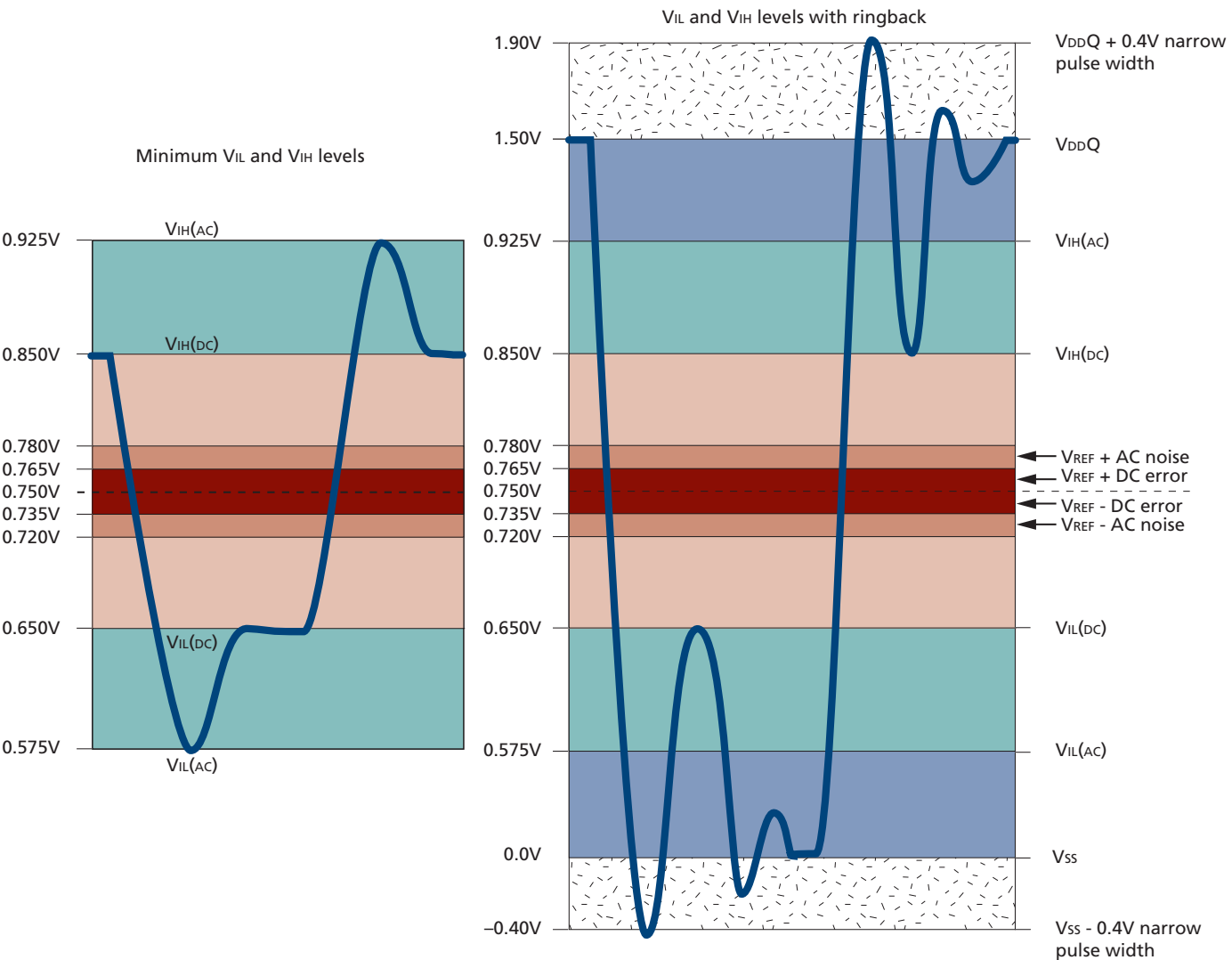
Figure 13: Input Signal
