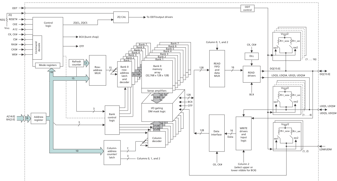
Figure 4: 256 Meg x 16 Functional Block Diagram
