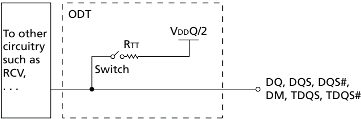
Figure 107: On-Die Termination
