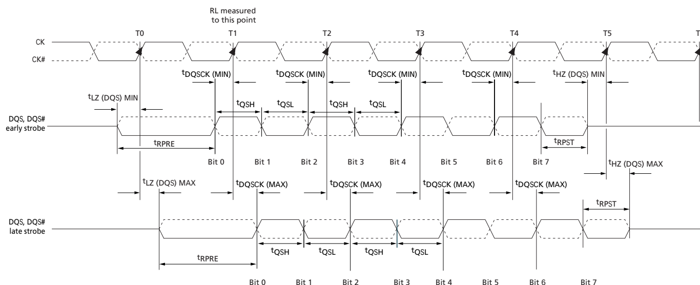
Figure 78: Method for Calculating t_{LZ} and t_{HZ}
