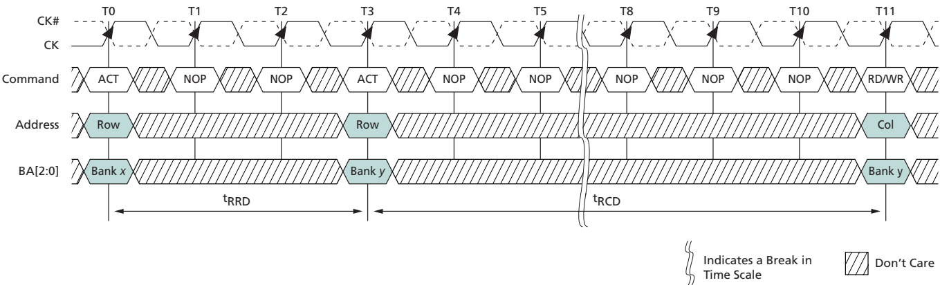
Figure 64: Example: Meeting t_{RRD}(\text{MIN}) and t_{RCD}(\text{MIN})
