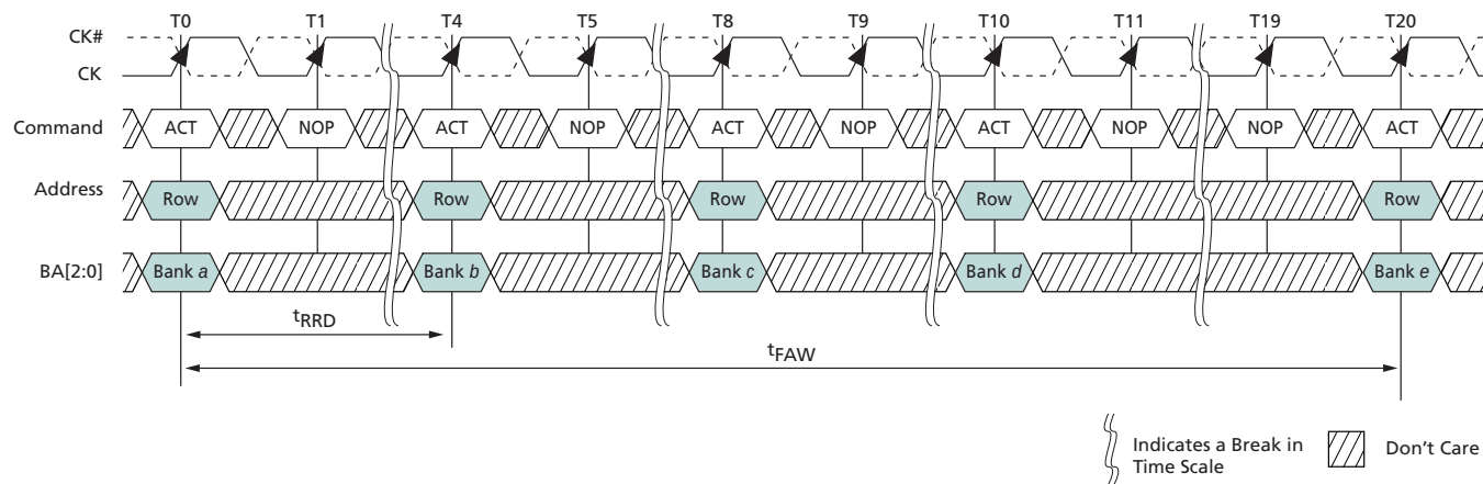
Figure 65: Example: t_{FAW}
