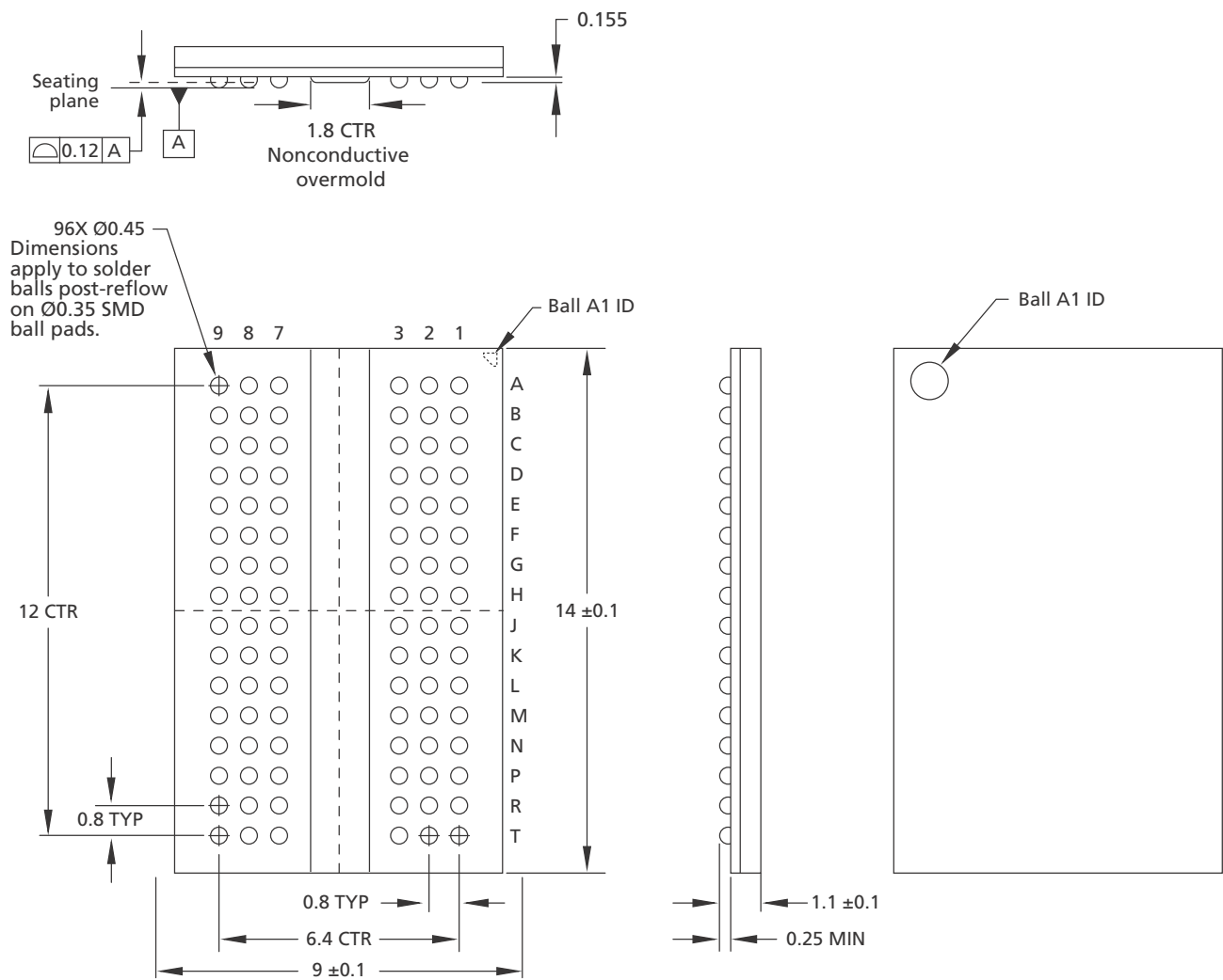
Figure 11: 96-Ball FBGA – x16; “GPF”
