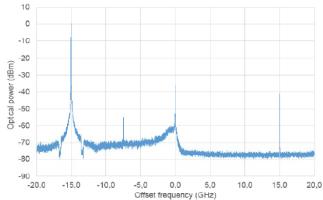
Optical CS-SSB modulation with carrier and subcarrier (modulation @15 GHz)
