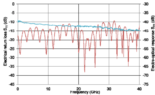
Typical Curve S_{21} & S_{11} from RF 2 Electrode
