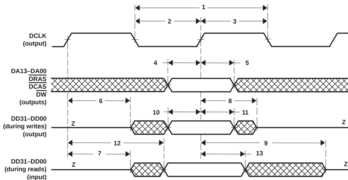
Figure 16. SDRAM Subcycle
