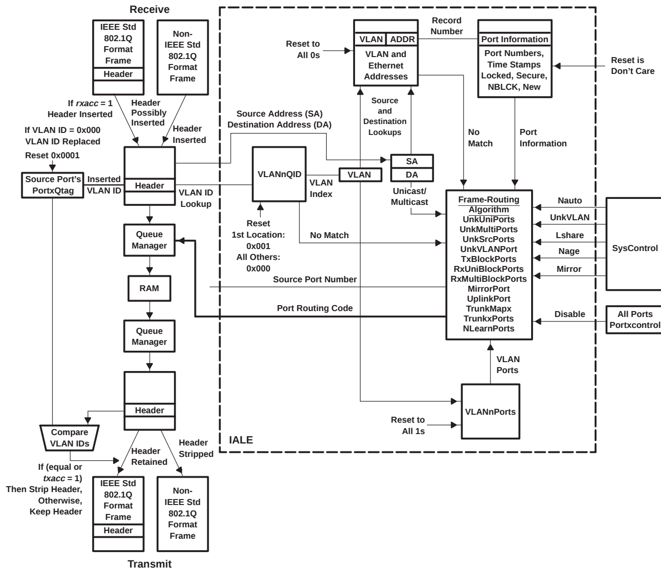
Figure 7. VLAN Overview
