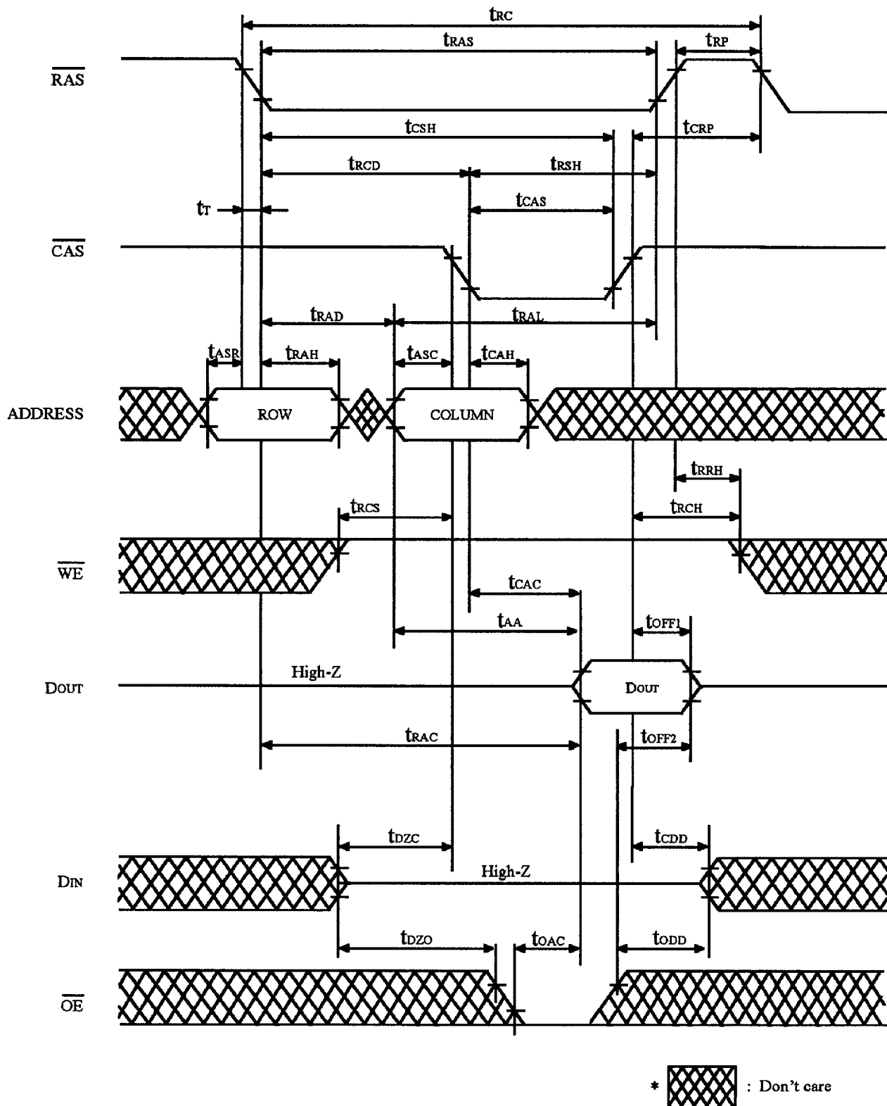
FIGURE 1. READ CYCLE
