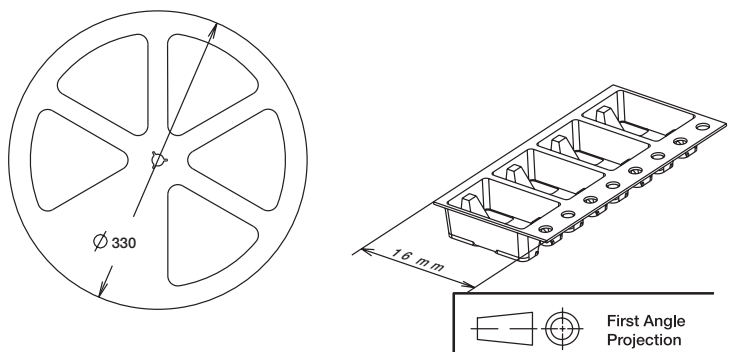
TAPE AND REEL KSC2G & KSC4
