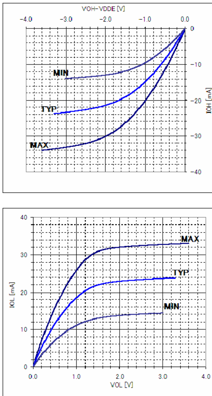
Fig. 9.3 3.3 V Standard CMOS I/O V-I Characteristic (Driving capability 1)
