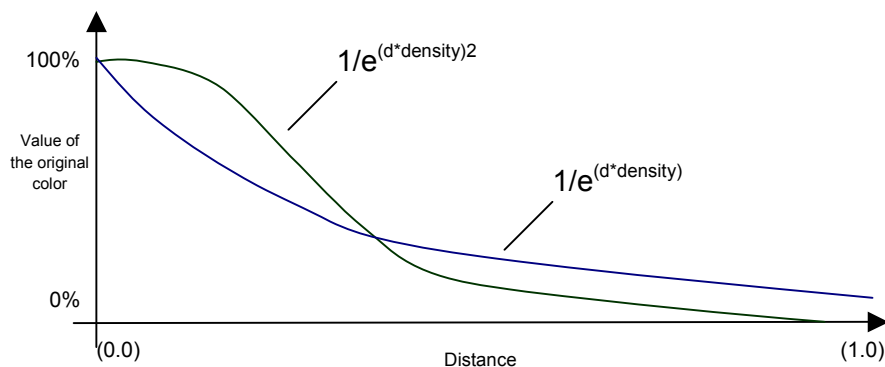
Fig. 6.16 Schematic Diagram of Fog Factor Table in OpenGL Mode
