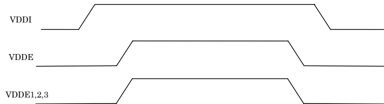
Fig. 9.1 Recommended Power ON/OFF Sequence (1)
