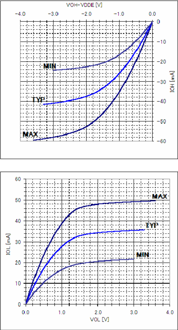
Fig. 9.4 3.3 V Standard CMOS I/O V-I Characteristic (Driving capability 2)
