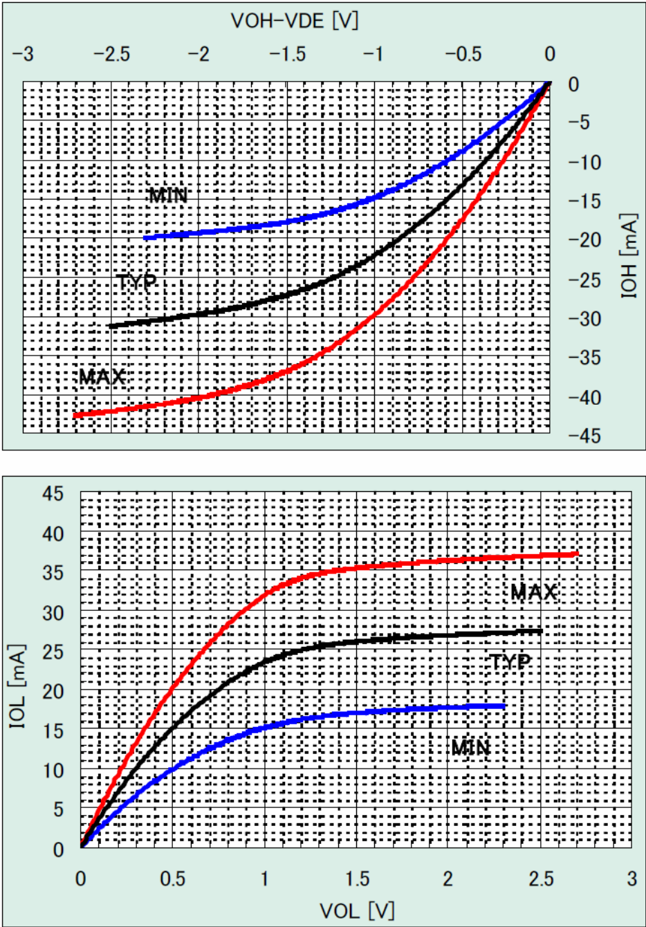
Fig. 9.7 2.5 V LVCMOS V-I Characteristic (Driving capability 1)
