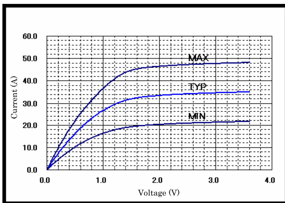
I 2 C IO V-1 Characteristic Figure
