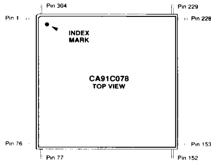
Figure 4.2 : Pin Configuration for 304-Pin PQFP Package
