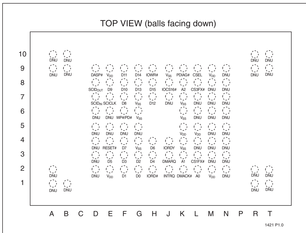
Figure 2: Pin Assignments for 91-Ball PBGA
