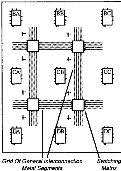
Figure 10. General Purpose Interconnections
