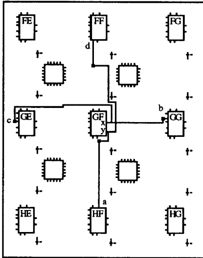
Figure 12. Direct Interconnection
