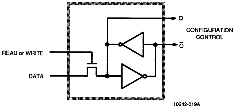
Figure 1. Basic Memory Cell
