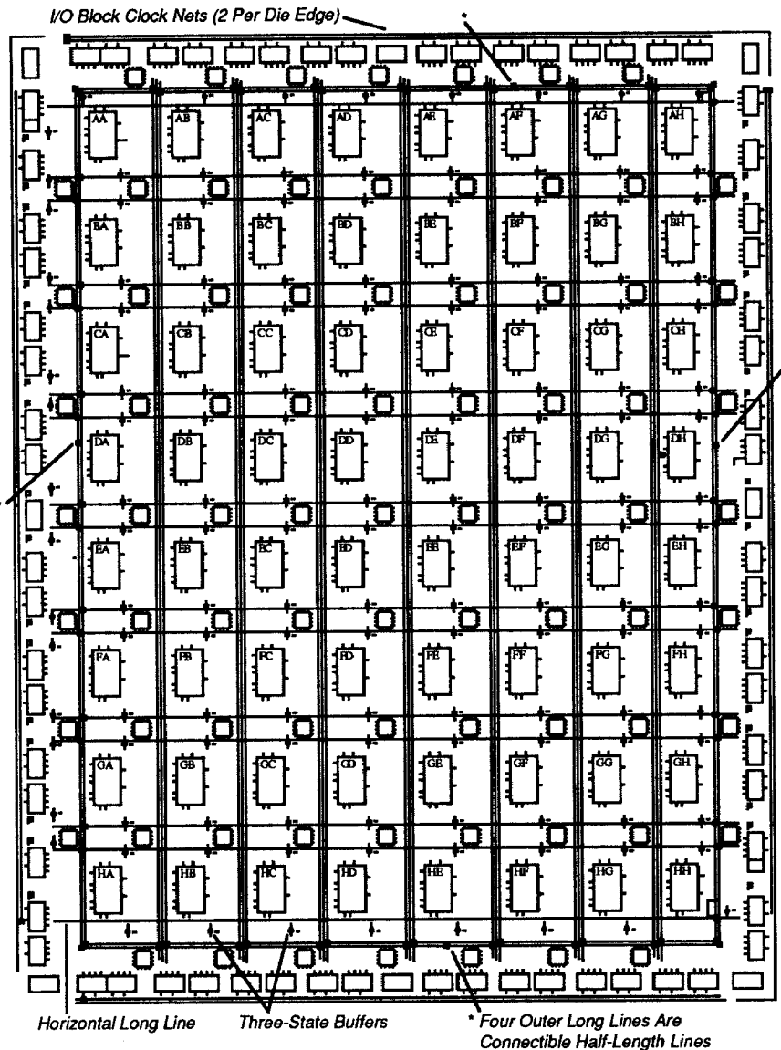
Figure 15. Interconnection of Long Lines
