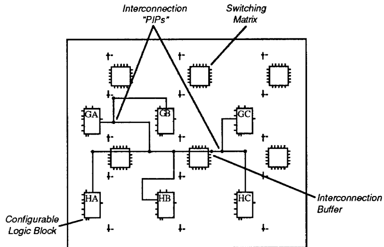
Figure 8. Routing Resources
