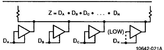
Figure 17. Three-State Buffers Implement a Wired-AND Function
