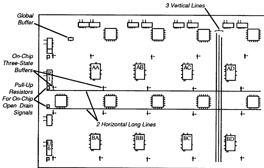
Figure 14. Long Lines
