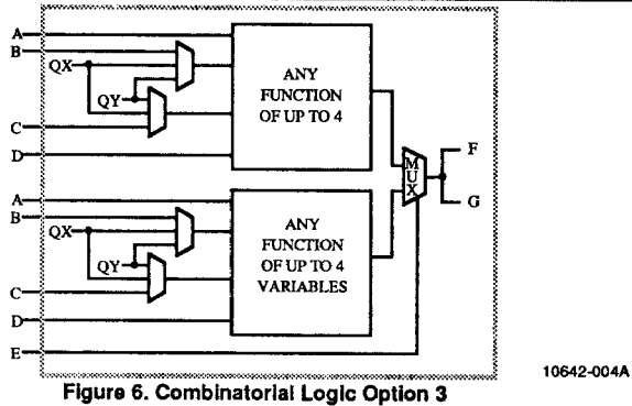
Figure 6. Combinatorial Logic Option 3
