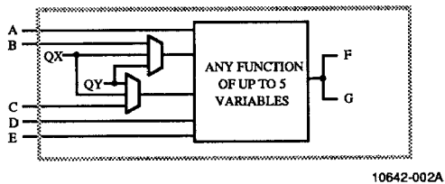
Figure 4. Combinatorial Logic Option 1
