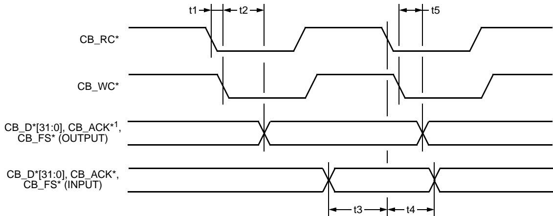
Figure 28. Cell Bus Timing
