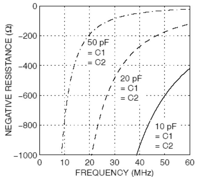
Figure 19. Negative Resistance Plot
