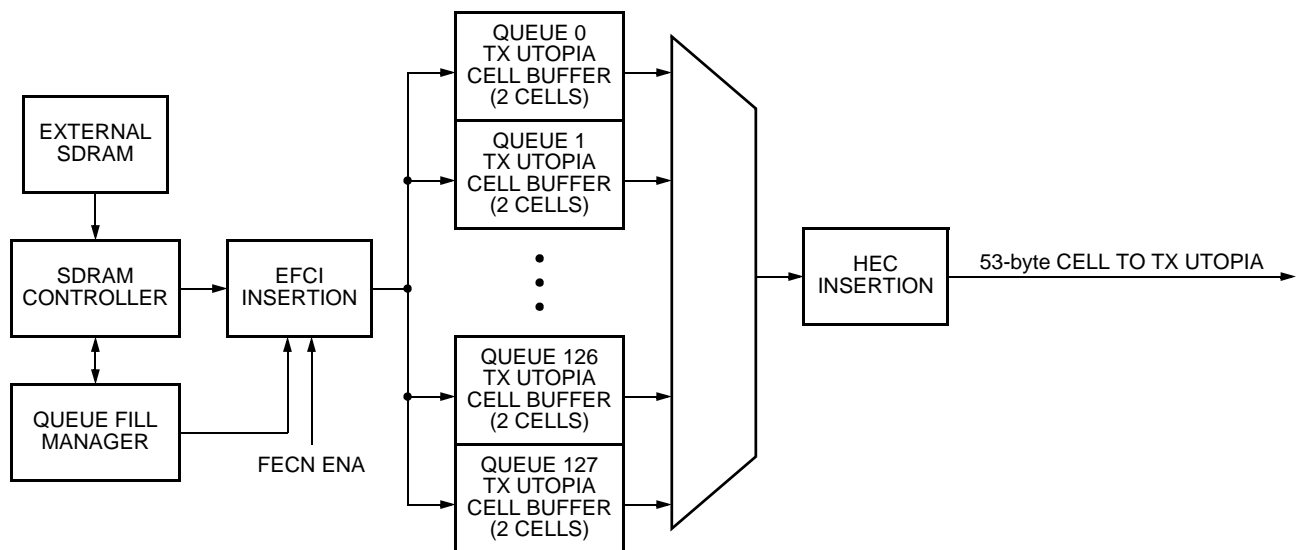
Figure 10. TX UTOPIA Cell Handling
