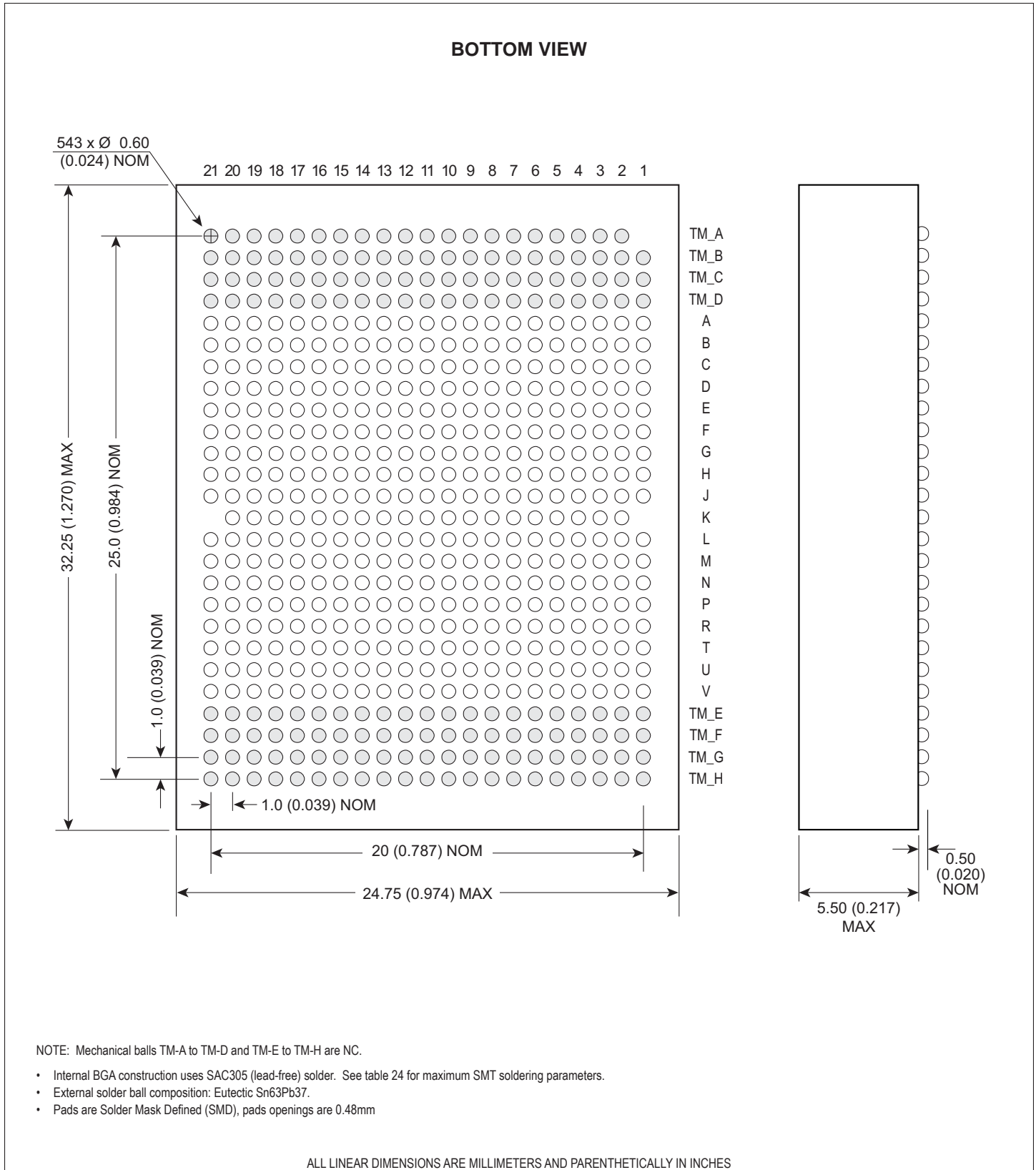
FIGURE 15 – PACKAGE DIMENSION: 543 PLASTIC BALL GRID ARRAY (PBGA) for W3J1G72K-XPBX
