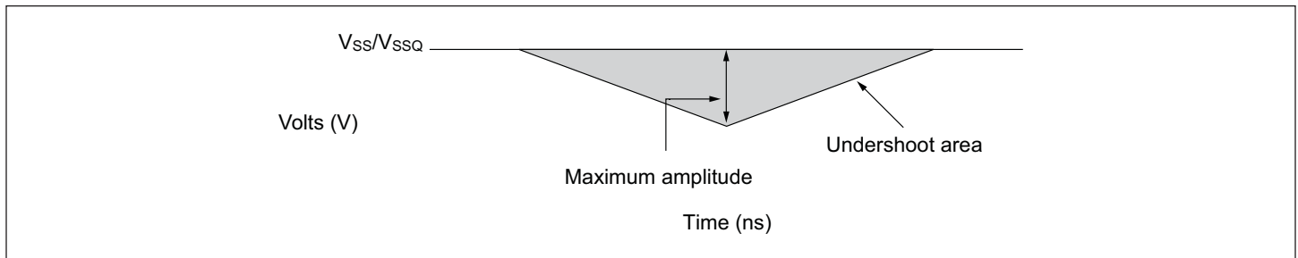
FIGURE 14 – UNDERSHOOT
