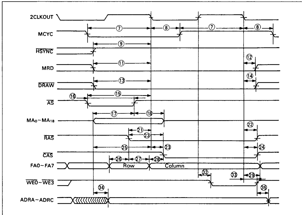
Figure 21. Memory Write Cycle
