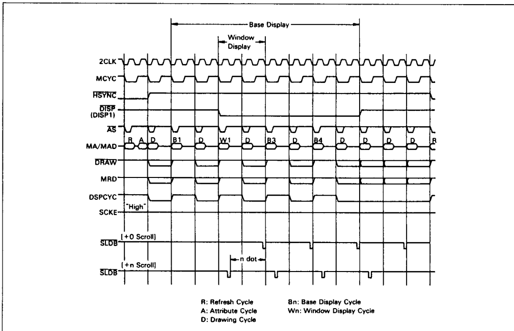
Figure 10. SLDB Timing (Dual Access Mode 0)
