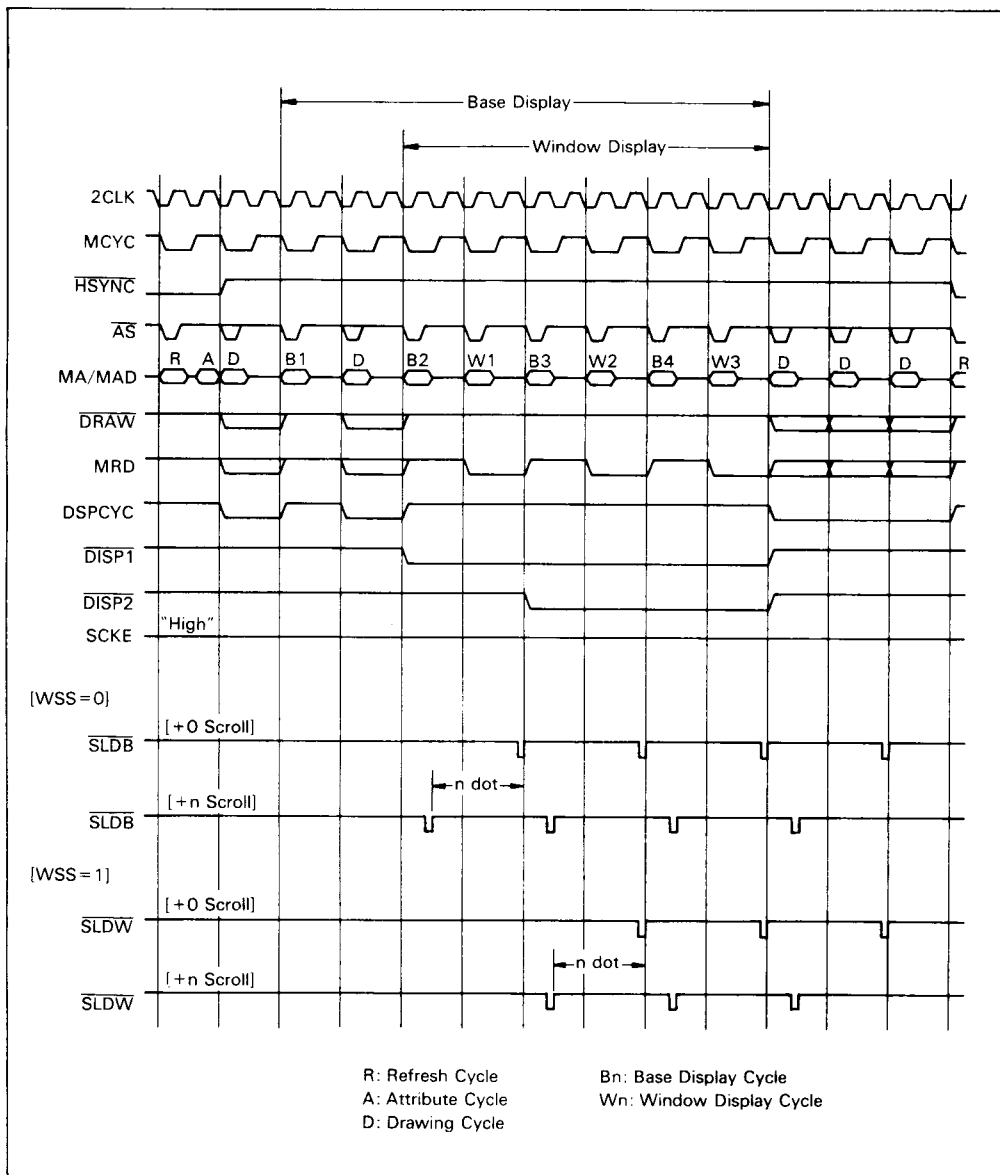
Figure 11. \overline{SLDB} and \overline{SLDW} Timing (Dual Access Mode 1)
