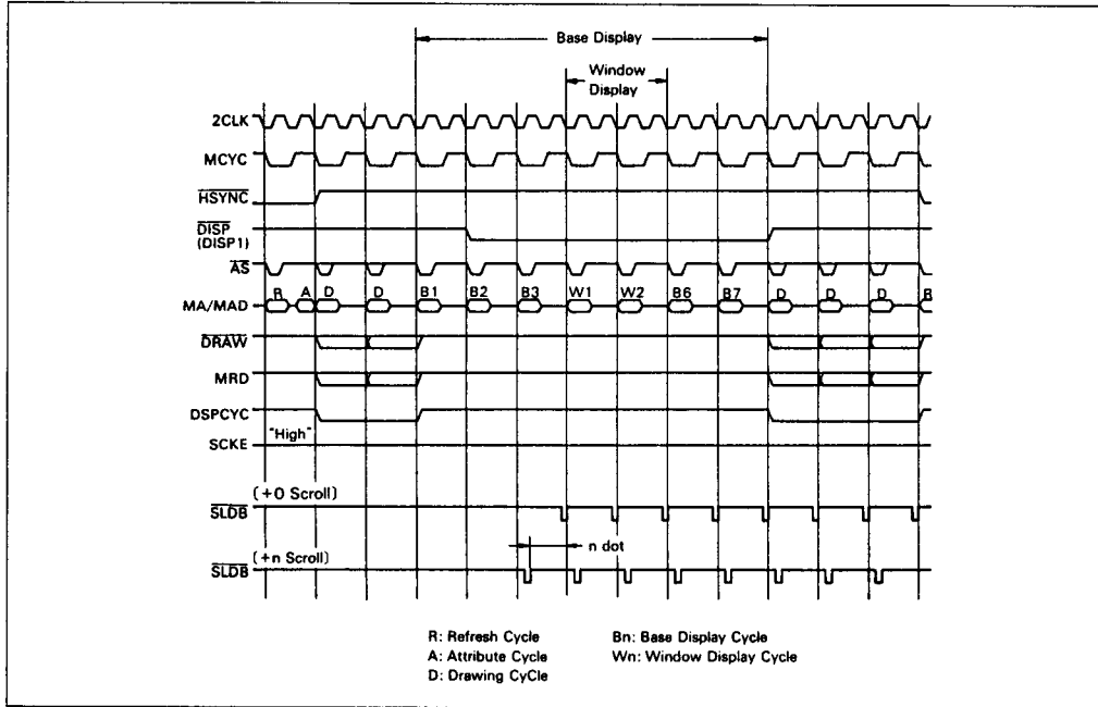
Figure 9. SLDB Timing (Single Access Mode)
