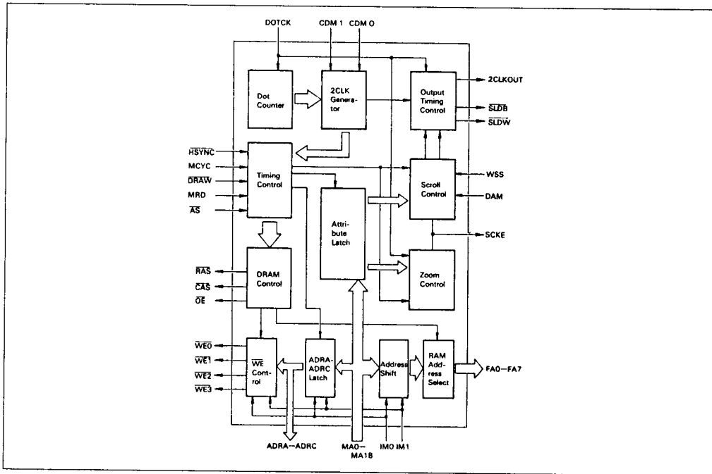
Figure 2. GMIC Block Diagram
