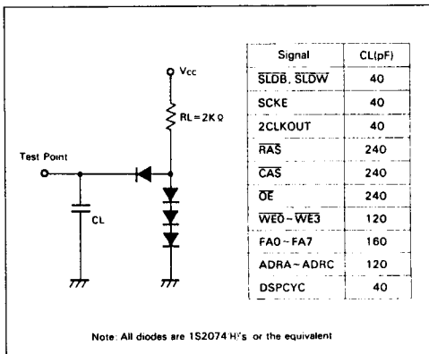
Figure 24. Test Load Circuit
