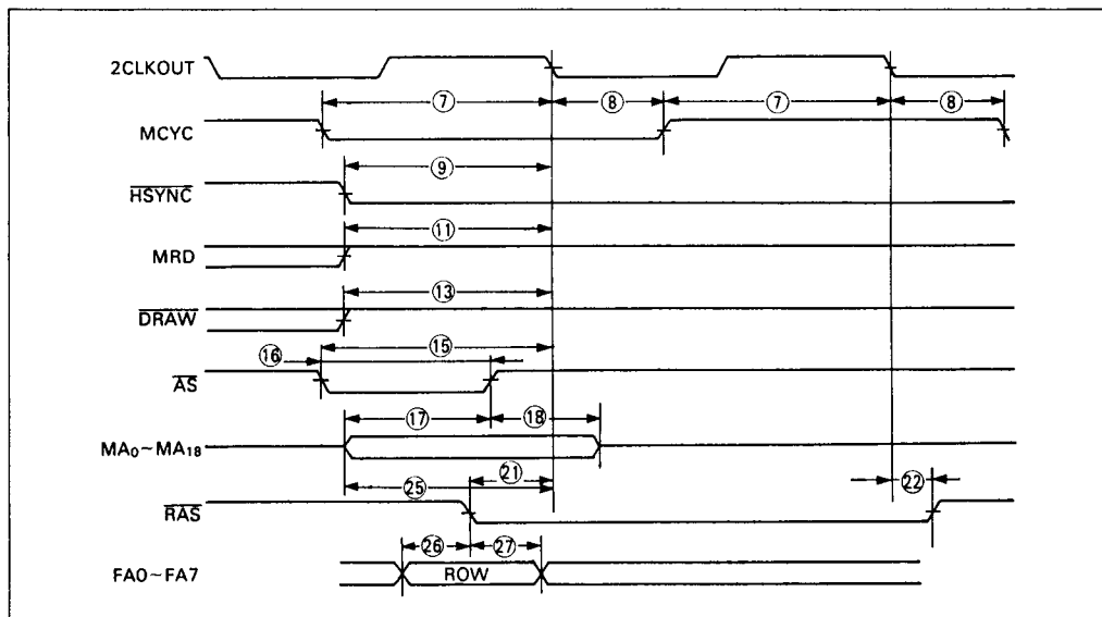
Figure 22. Refresh Cycle
