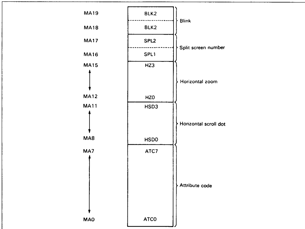
Figure 17. Attribute Control Signal Output Pins
