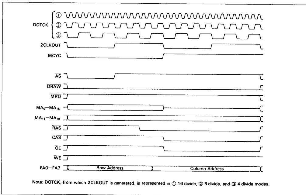
Figure 6. Read Cycle Timing
