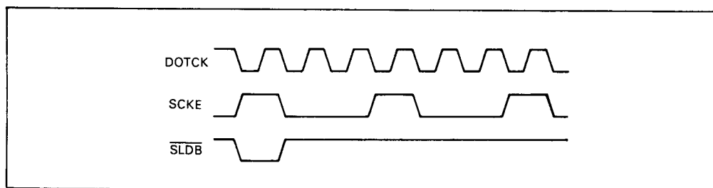
Figure 15. Triple Zoom Timing
