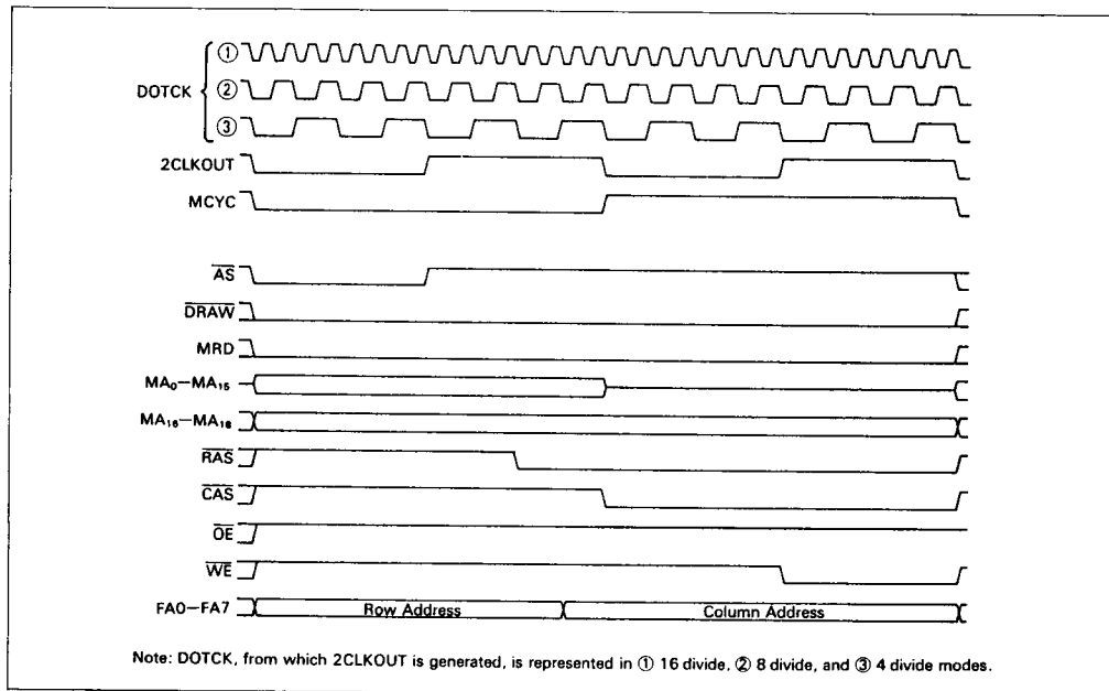
Figure 7. Write Cycle Timing
