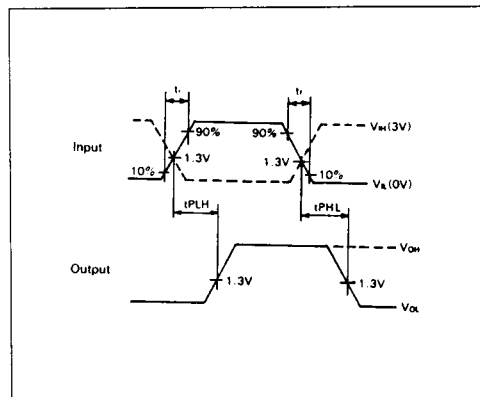
Figure 25. Input/Output Waveforms
