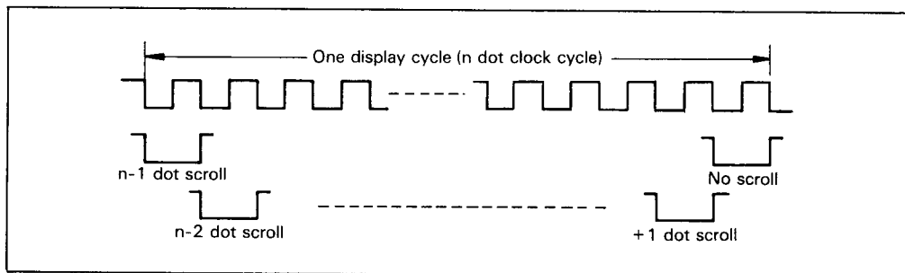
Figure 8. Shift Load ( \overline{SLDB} , \overline{SLDW} ) Output Timing
