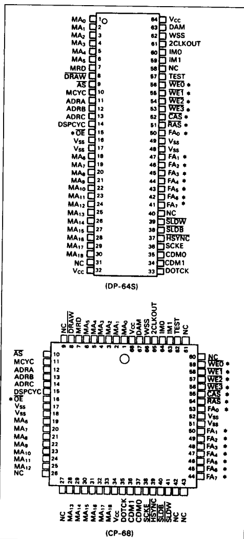
Figure 1. Pin Arrangement
