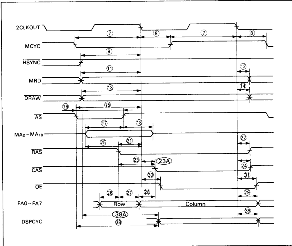
Figure 20. Memory Read Cycle (Drawing Read and Display)
