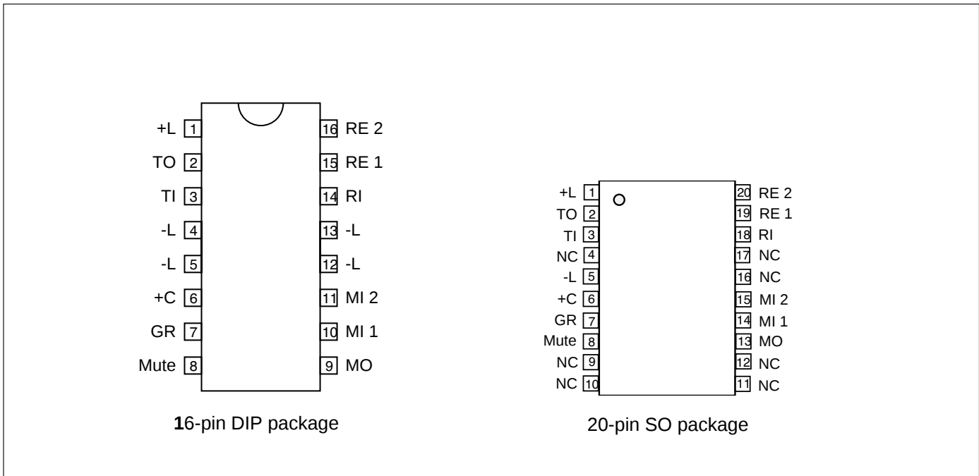
Figure 8. Pin configuration,16 -pin DIP and 20-pin SO package.
