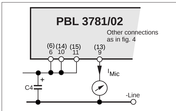
Figure 5. Microphone amplifier used as a DC-current supply.
