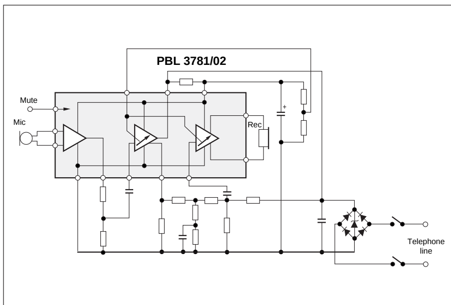
Figure 1. Functional diagram.
