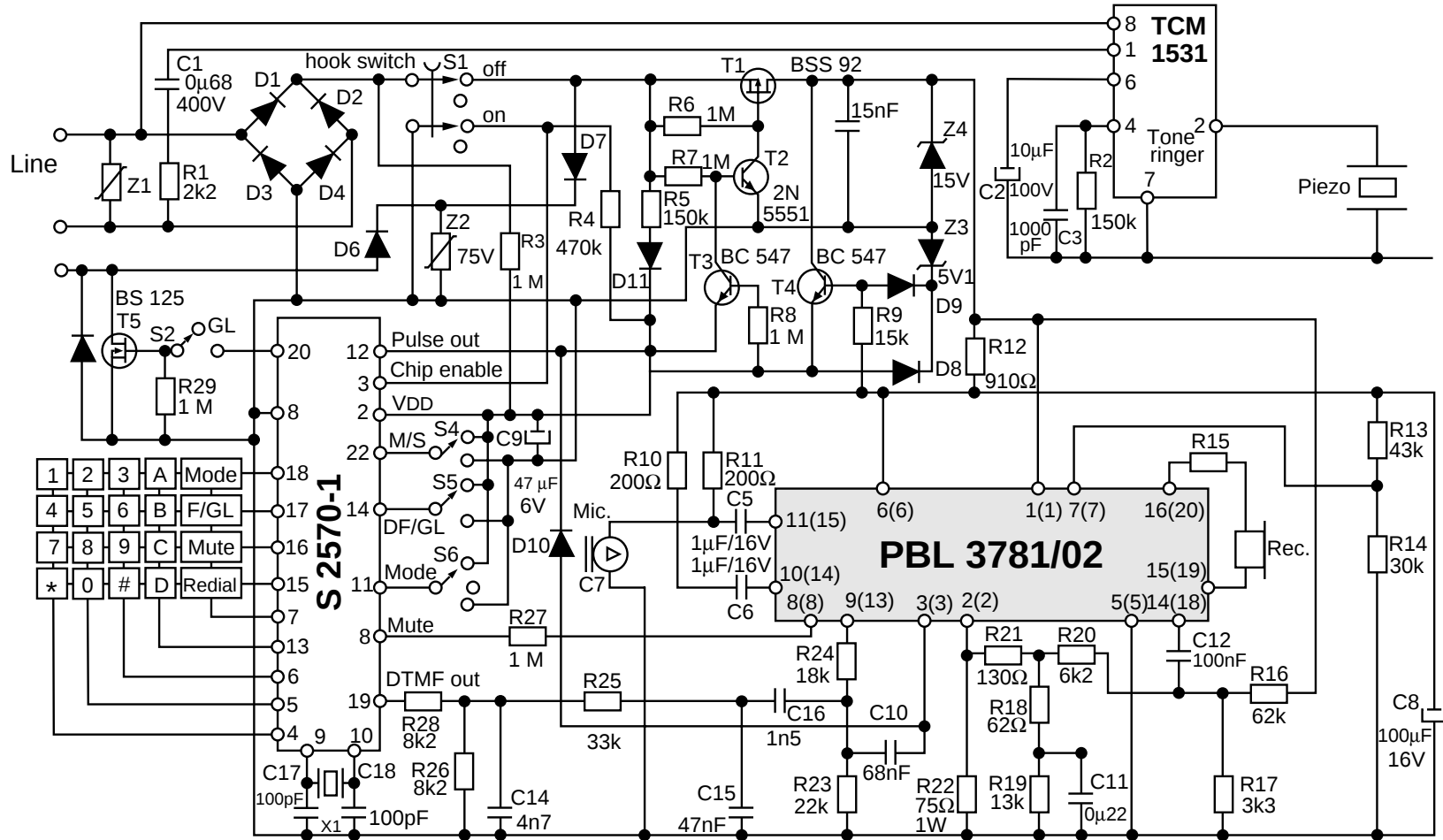
Figure 15. Typical tone-dialing telephone for 48V 2 x 400 \Omega battery feeding system.
