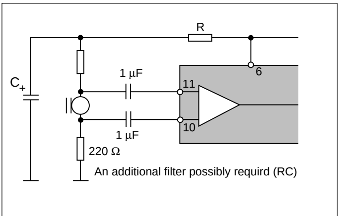
Figure 11. Balanced electret microphone connection.
