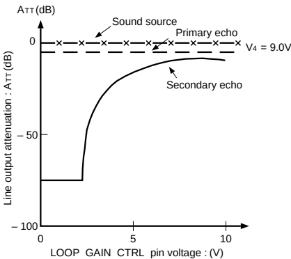
Line output attenuation vs. loop gain control pin voltage
