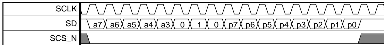
Figure 5-20 SPI power_stream (spi_clock_polarity = 1, rising edge of SCLK is active)
