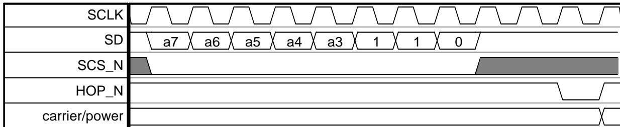
Figure 5-23 SPI hop_stream (spi_clock_polarity = 0, falling edge of SCLK is active)
