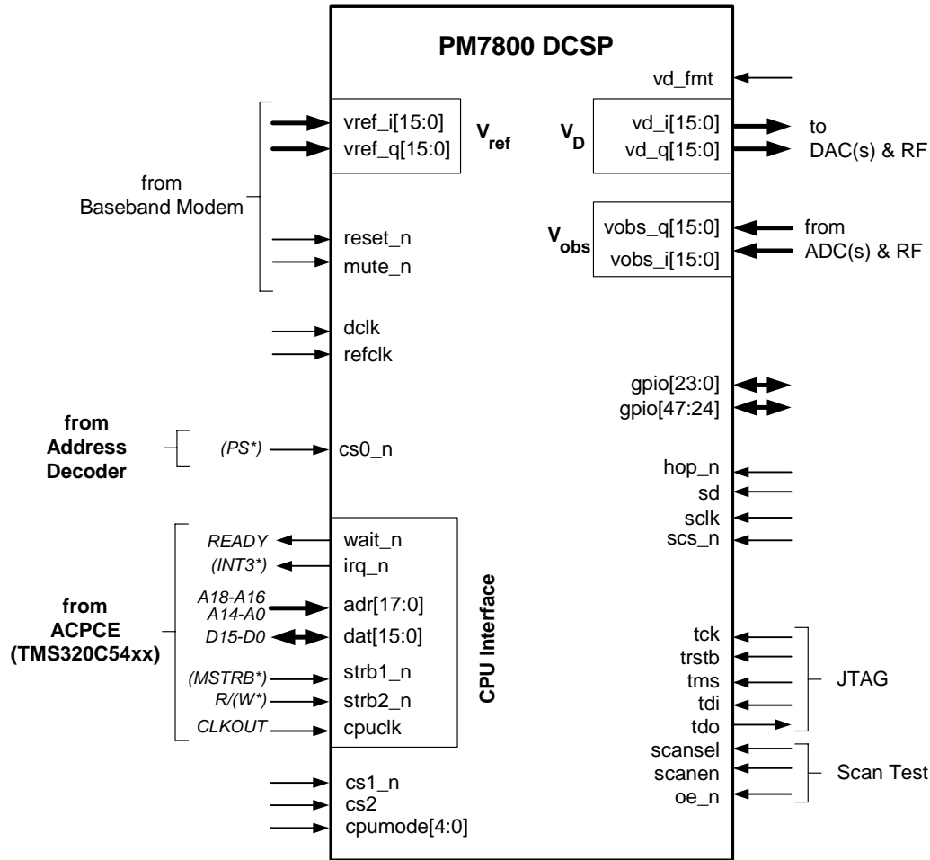
Figure 2-1 PM7800 Block Diagram
