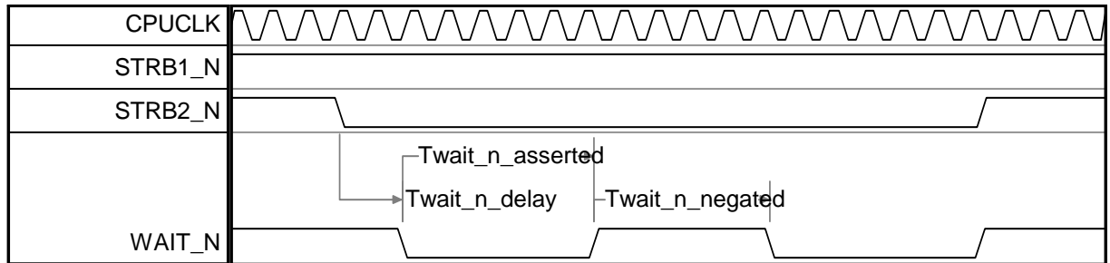
Figure 5-9 WAIT_N Timing - Reads (CPUMODE0 = 1)
