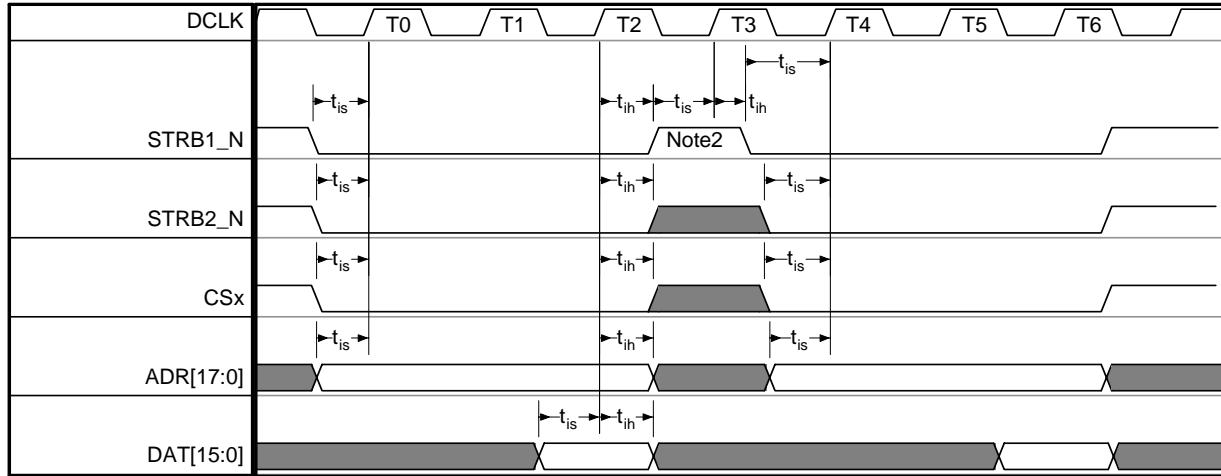
Figure 5-6 Back-to-Back Write Cycles (CPUMODE0 = 0)
