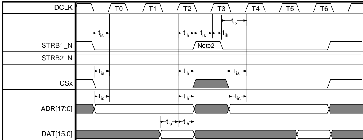
Figure 5-7 Back-to-Back Write Cycles (CPUMODE0 = 1)
