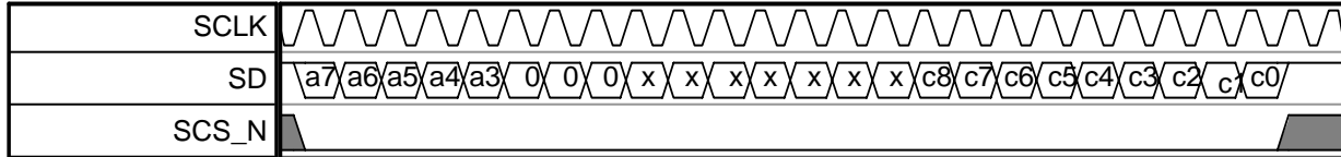
Figure 5-18 SPI carrier_stream (spi_clock_polarity = 1, rising edge of SCLK is active)
