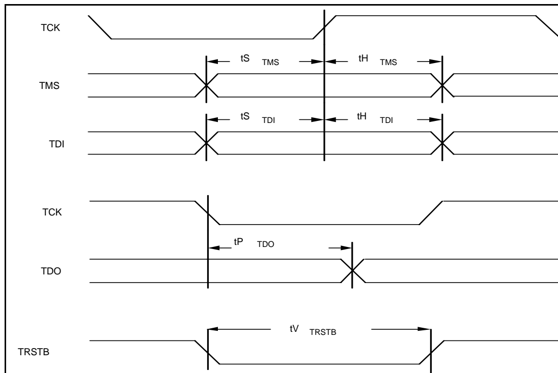
Figure 9-8 JTAG Interface
