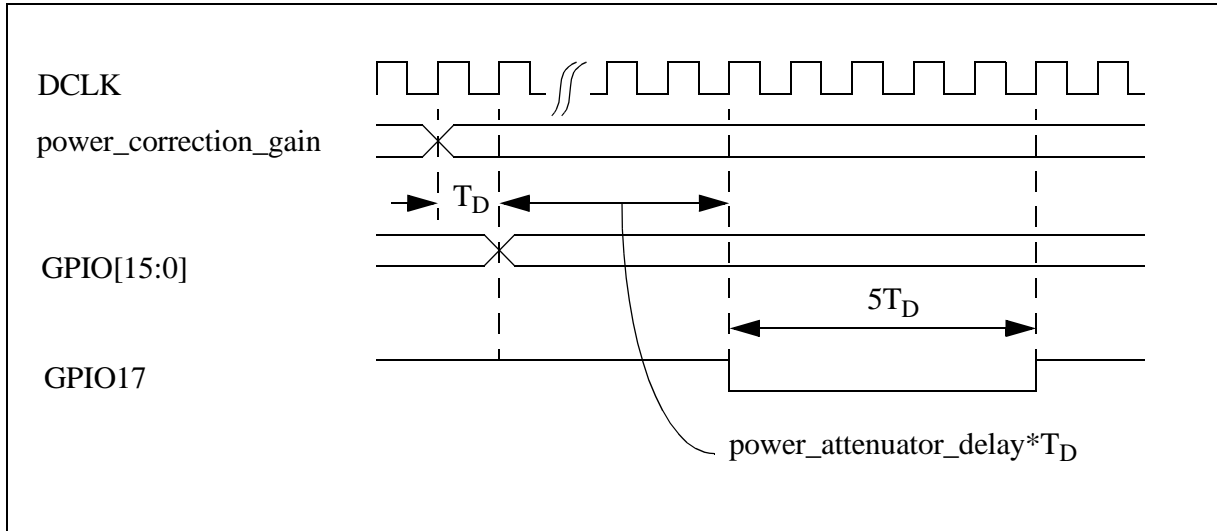
Figure 5-25 Power Attenuator Outputs - shown with active-low pulse on GPIO17
