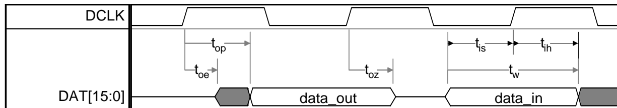
Figure 9-7 GPIO
