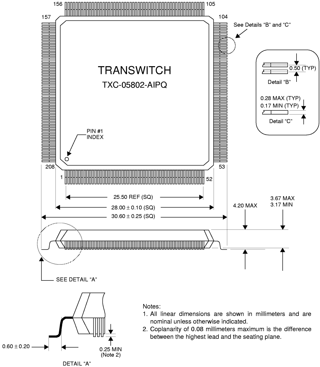
Figure 55. CUBIT-Pro TXC-05802 208-Pin Plastic Quad Flat Package
