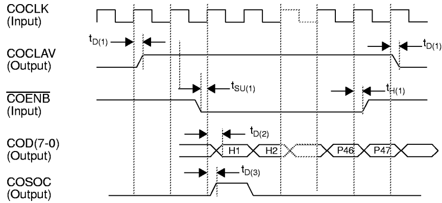
Figure 46. Timing of Back-to-Back Cell Transmit Interface
