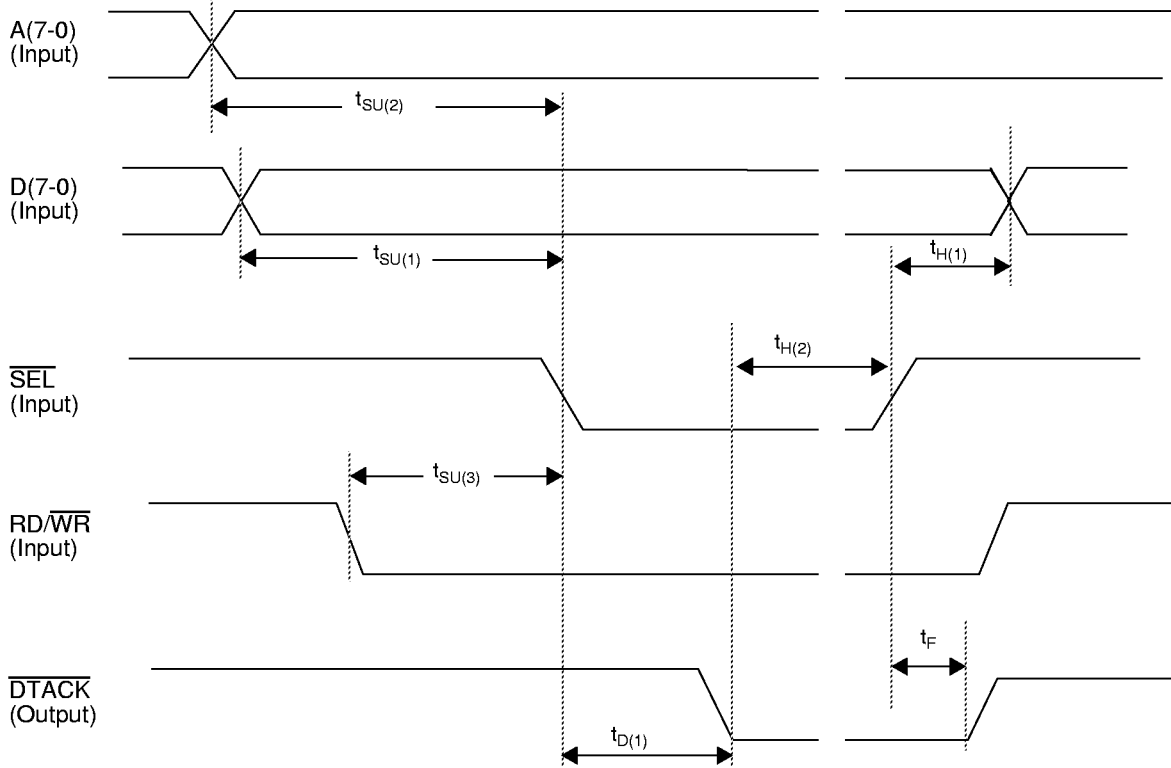
Figure 53. Motorola Microprocessor Write Cycle Timing
