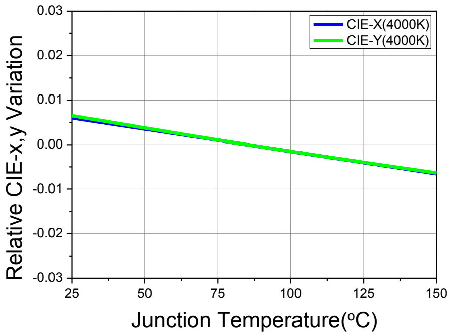
Fig 9. Junction Temperature vs. CIE x,y Shift, I_f=0.18A (CRI80, 4000K)
