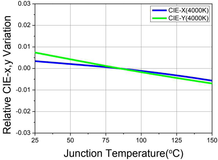
Fig 11. Junction Temperature vs. CIE x,y Shift, I_f=0.18A (CRI90, 4000K)
