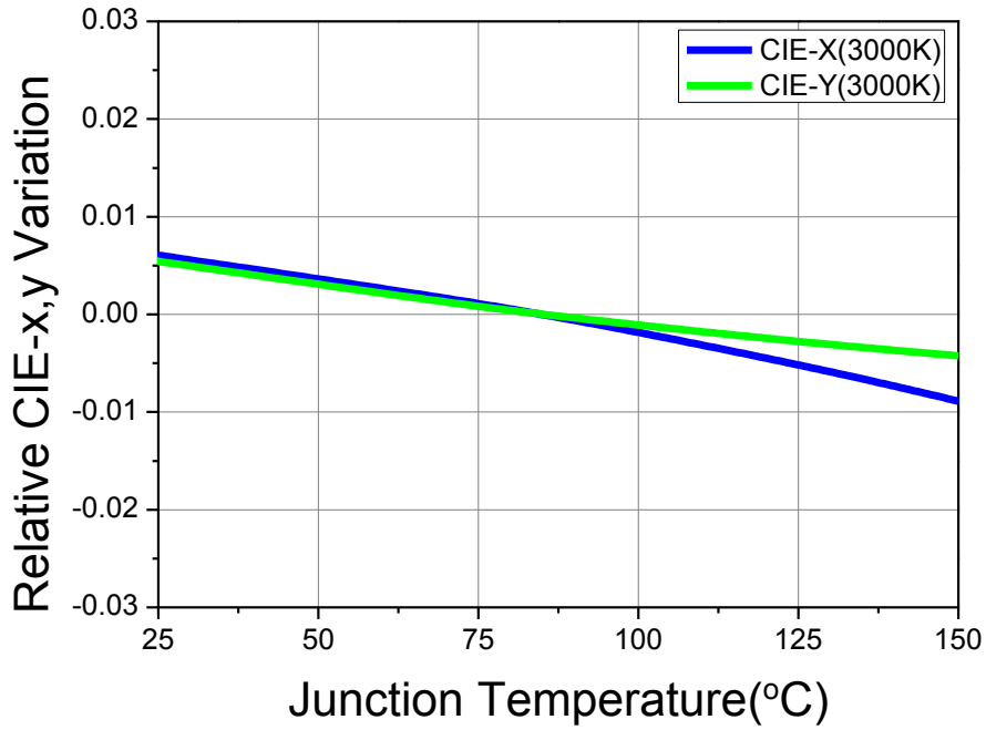
Fig 10. Junction Temperature vs. CIE x,y Shift, I_f=0.18A (CRI80, 3000K)
