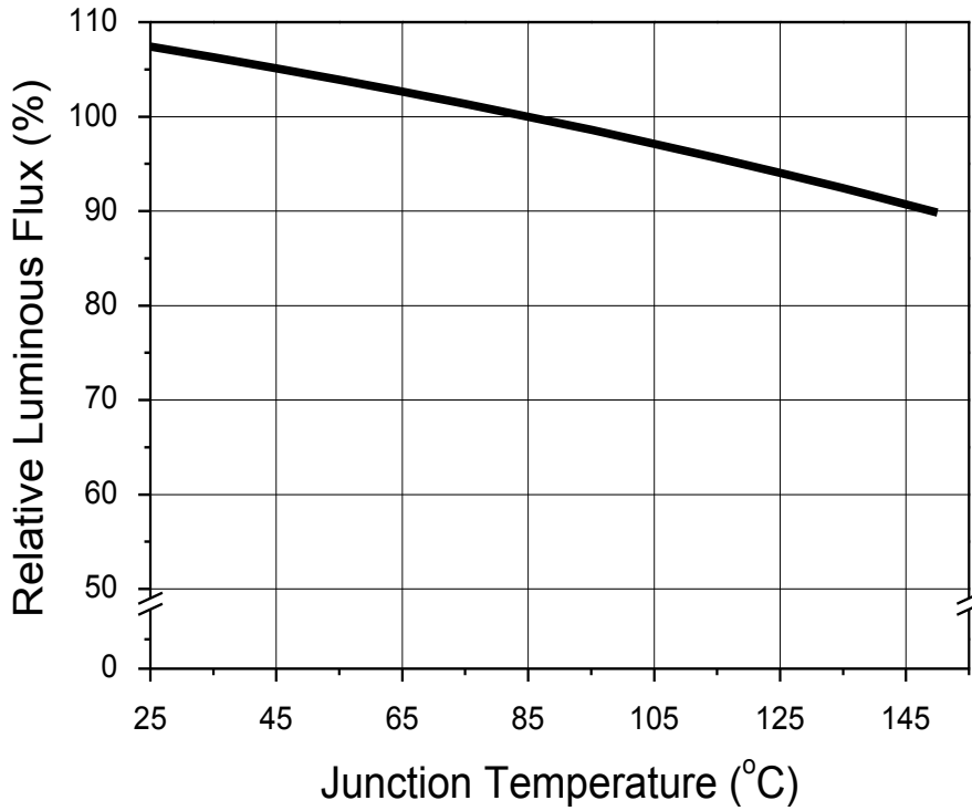
Fig 6. Junction Temperature vs. Relative Luminous Flux, I_F=0.18A
