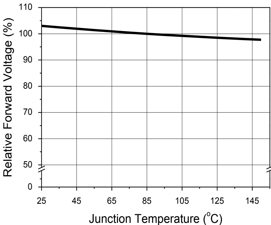
Fig 7. Junction Temperature vs. Forward Voltage, I_F=0.18A
