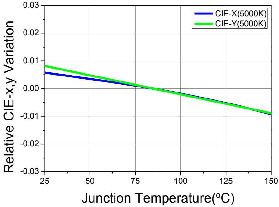
Fig 8. Junction Temperature vs. CIE x,y Shift, I_f=0.18A (CRI80, 5000K)
