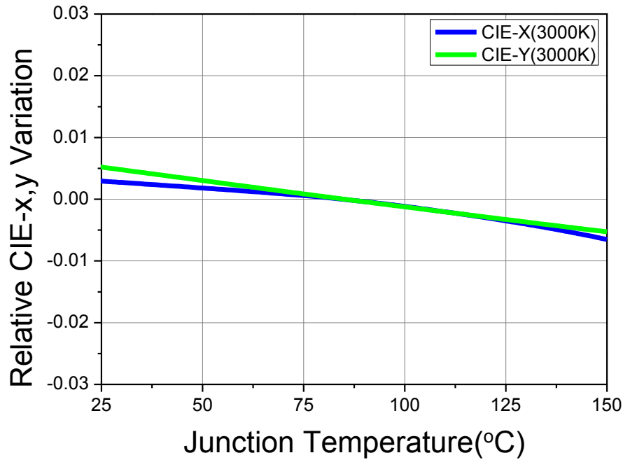
Fig 12. Junction Temperature vs. CIE x,y Shift, I_f=0.18A (CRI90, 3000K)
