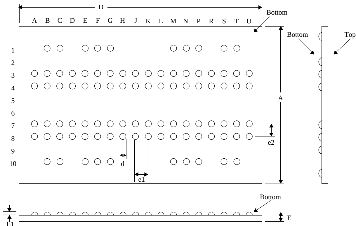
Figure 4: Center-Bonded uBGA Package
