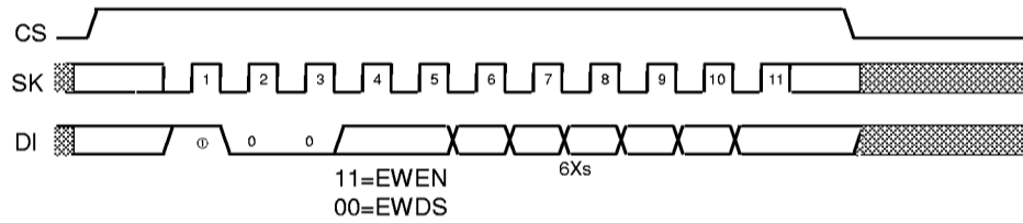
Figure 15 EWEN/EWDS Timing (S-29U331A)
