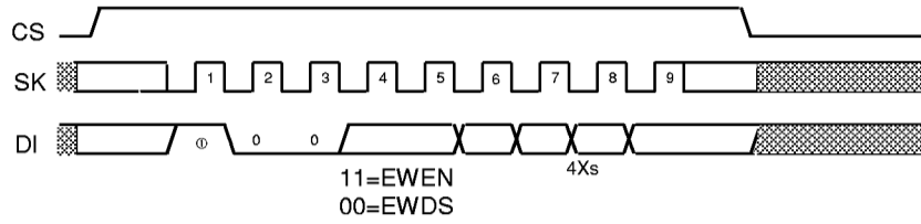
Figure 13 EWEN/EWDS Timing (S-29U131A)
