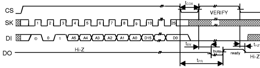
Figure 7 WRITE Timing (S-29U131A)
