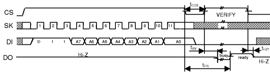
Figure 12 ERASE Timing (S-29U331A)
