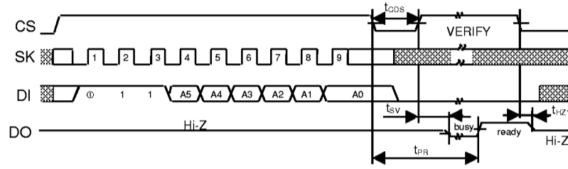
Figure 10 ERASE Timing (S-29U131A)
