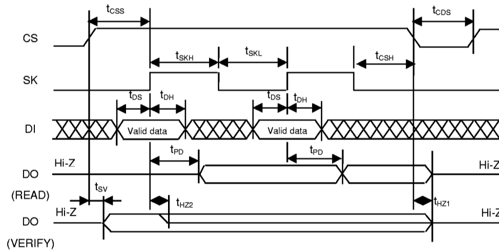
Figure 3 Timing Chart
