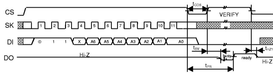
Figure 11 ERASE Timing (S-29U221A)
