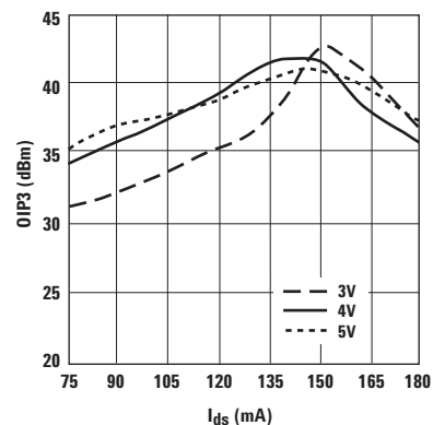
Figure 10. OIP3 vs. I_{ds} and V_{ds} at 3.9 GHz.
