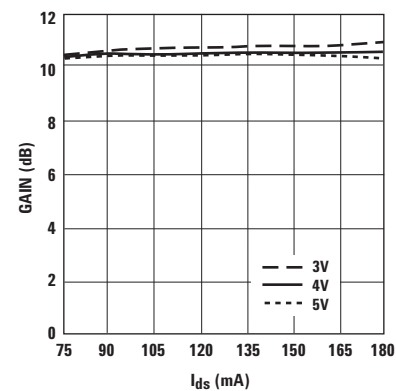
Figure 13. Small Signal Gain vs. I_{ds} and V_{ds} at 3.9 GHz.
