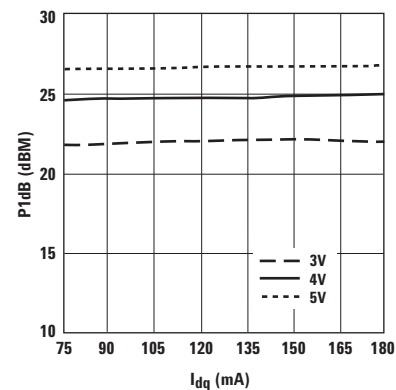
Figure 16. P1dB vs. I_{dq} and V_{ds} at 3.9 GHz.
