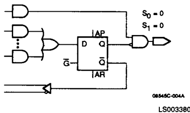
Figure 3-1. Latched/Active-LOW
