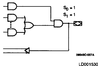
Figure 3-4. Combinatorial/Active-HIGH
