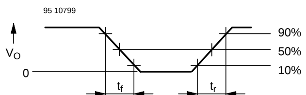
Figure 2. Pulse diagram
