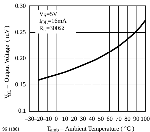
Figure 7. Output Voltage vs. Ambient Temperature
