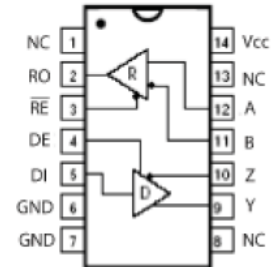
14-Pin PDIP/nSOIC
