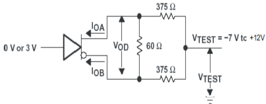
Figure 2. Driver Test Circuit, VOD With Common-Mode Loading
