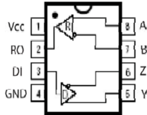
8-Pin PDIP/nSOIC/ MSOP
