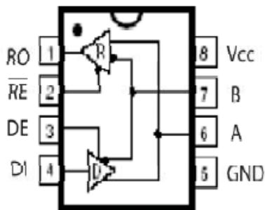
8-Pin PDIP/nSOIC/ MSOP
