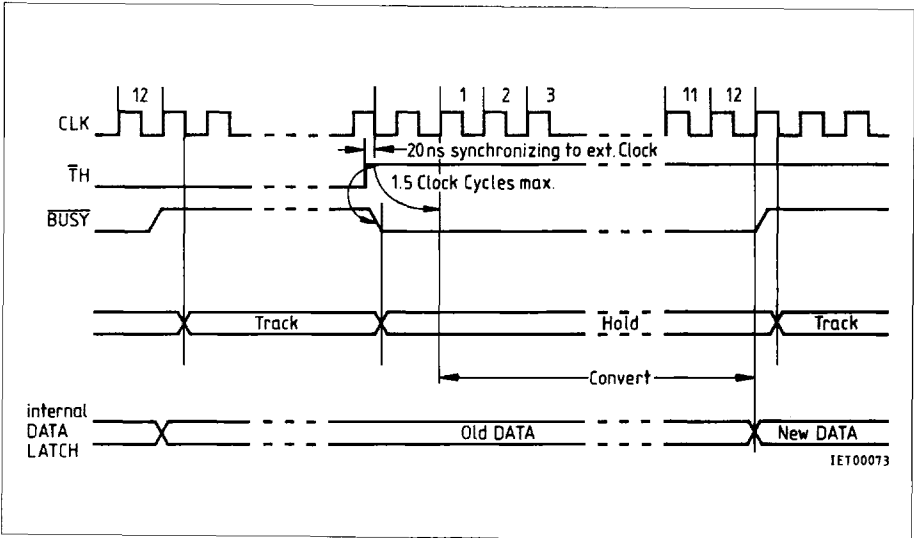
Figure 2 Starting a Conversion with TH (SDA 1812 D)
