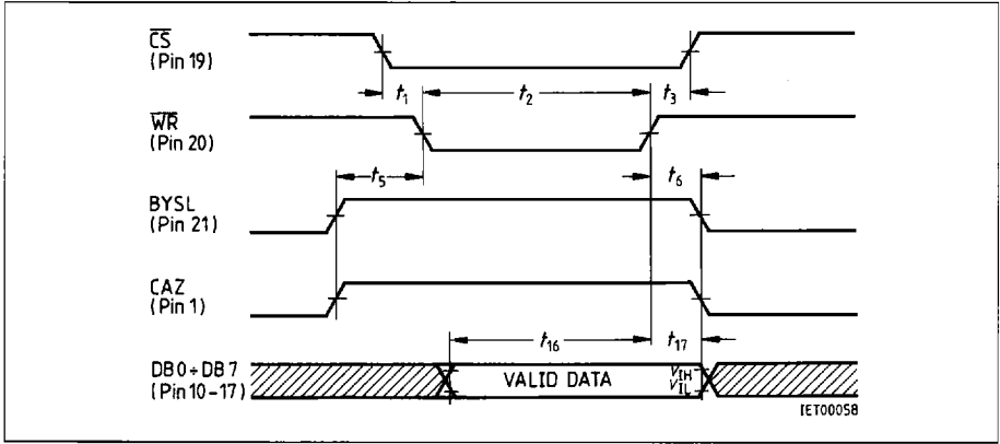
Figure 9 Writing to the SFR
