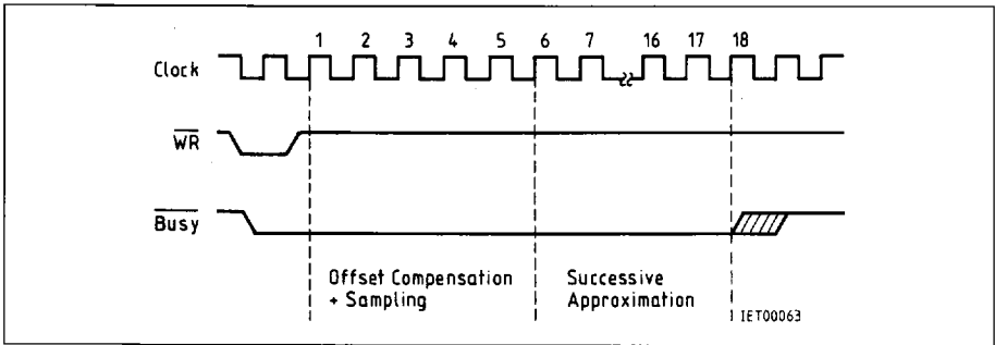
Figure 12 Converter Timing (SDA 0812 A)
