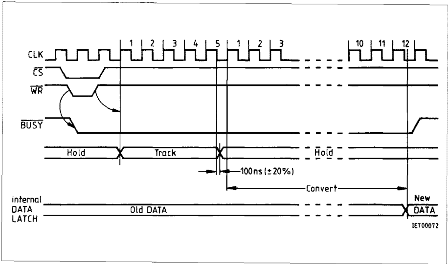
Figure 1 Starting a Conversion with WR
