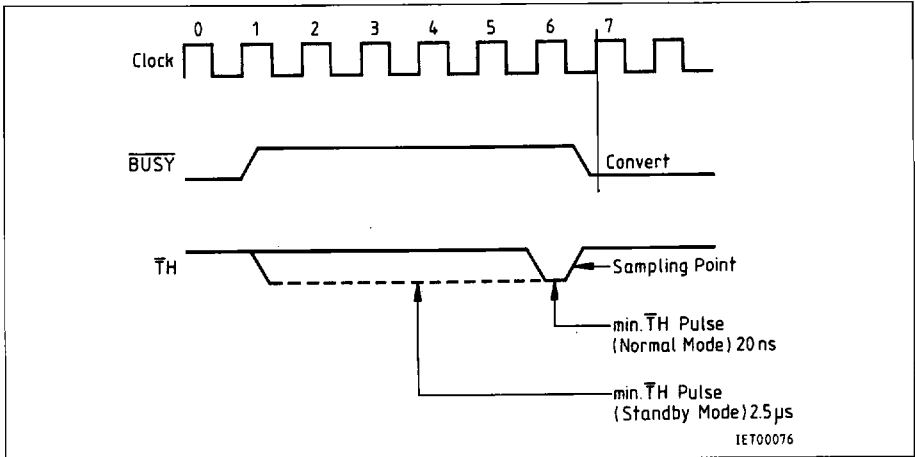
Figure 14 \overline{TH} -Timing (SDA 1812 D)
