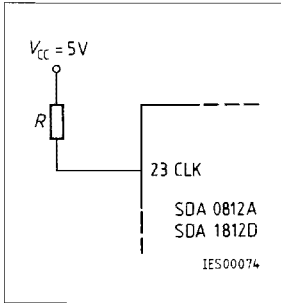
Figure 3 The Internal Clock Frequency only depends on the R Value
