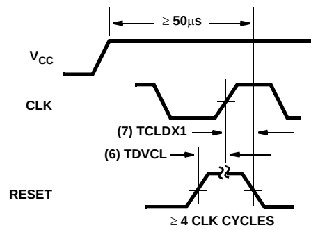
FIGURE 13. RESET TIMING
