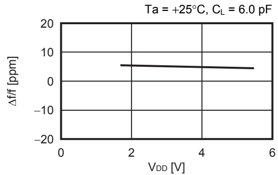
4. Crystal oscillator frequency deviation vs. Power supply voltage characteristics
