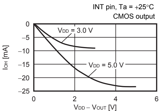
7. High level output current vs. VDD - VOUT characteristics
