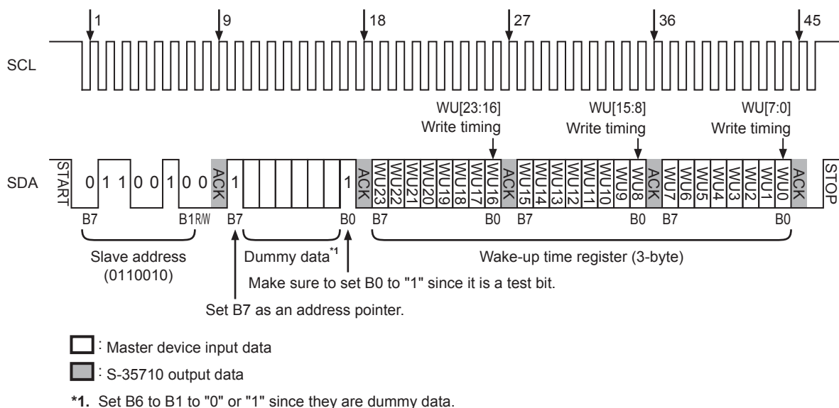
Figure 28 Write Timing of Wake-up Time Register SII Semiconductor Corporation
