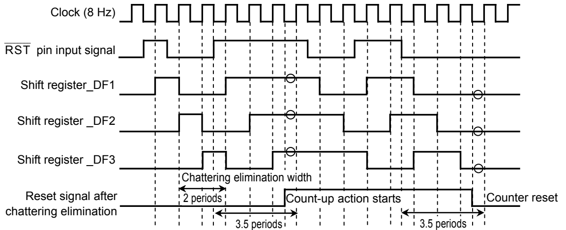
Figure 34 Timing Chart of Chattering Elimination
