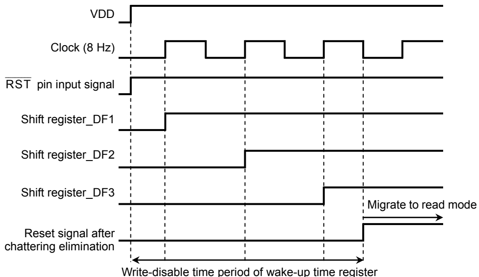
Figure 35 Timing Chart at Power-on
