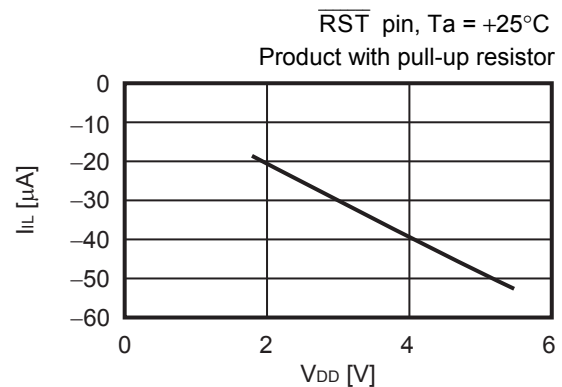
8. Low level input current vs. Power supply voltage characteristics
