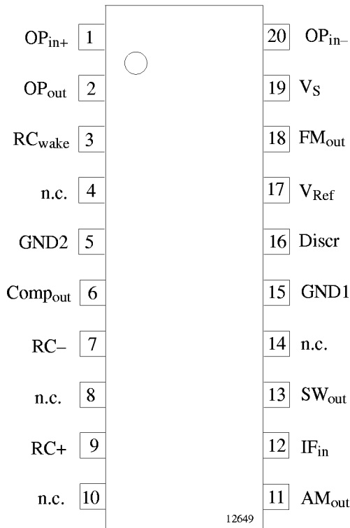
Figure 2. Pinning
