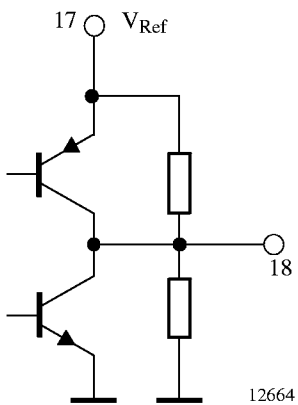
Figure 17. Pin 18 FM_{out}
