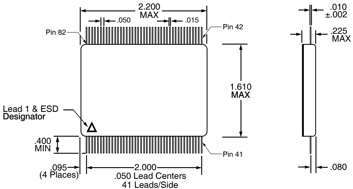
FIGURE 24 – FLAT PACKAGE OUTLINE (FP)
