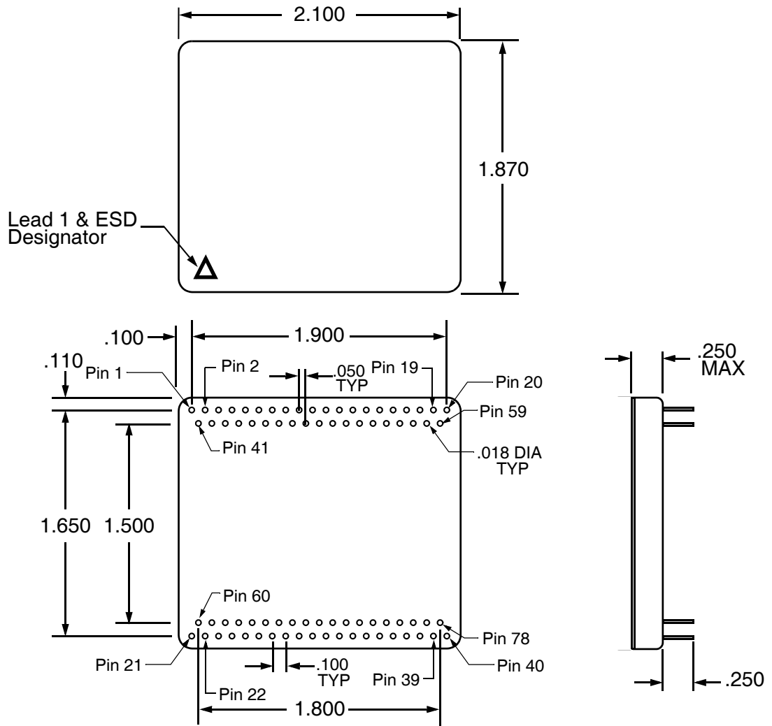
FIGURE 23 – PLUG IN PACKAGE OUTLINE (DIP)
