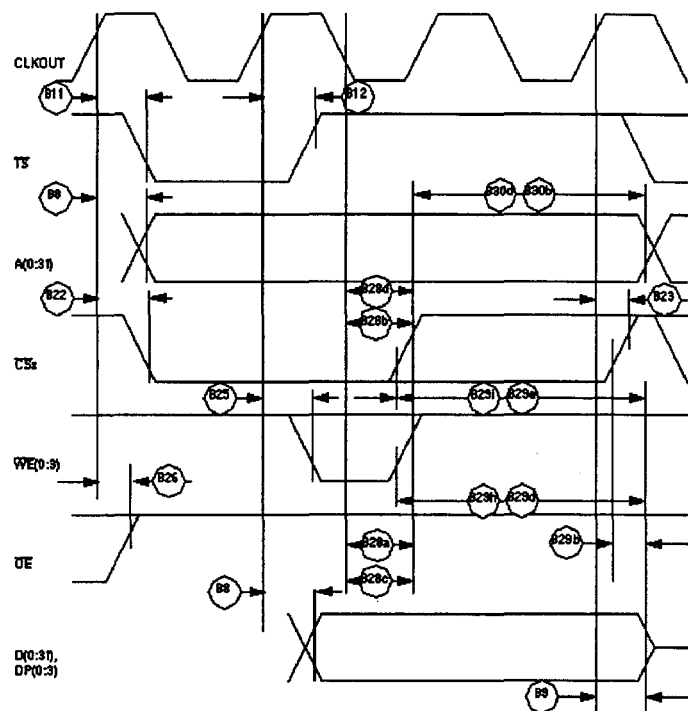
Figure 20 : External Bus Write Timing (GPCM controlled – TRLX = '1', CSNT = '1')
