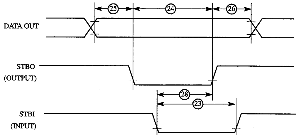
Figure 44 : PIP TX (Interlock Mode) Timing Diagram
