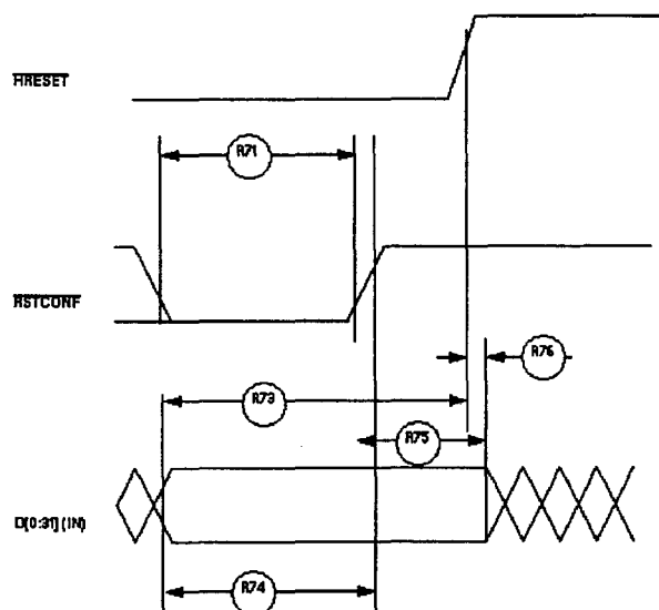
Figure 36 : Reset Timing – Configuration from Data Bus
