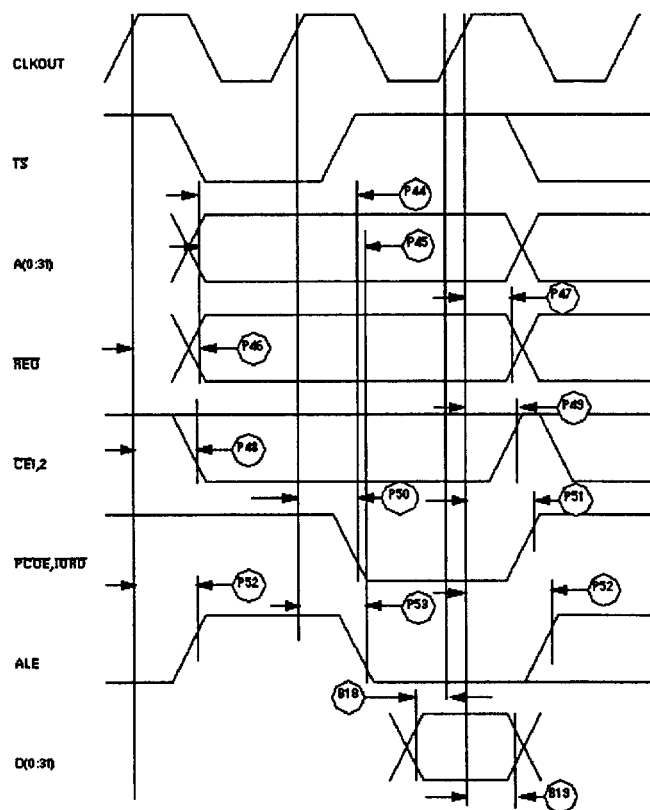
Figure 29 : PCMCIA access cycles Timing External Bus Read
