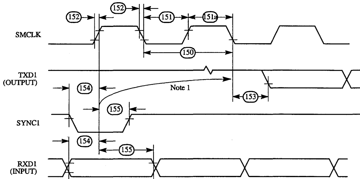
Figure 64 : SMC Transparent Timing Diagram
