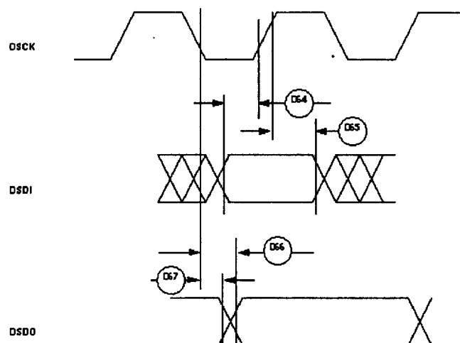
Figure 35 : Debug Port Timings
