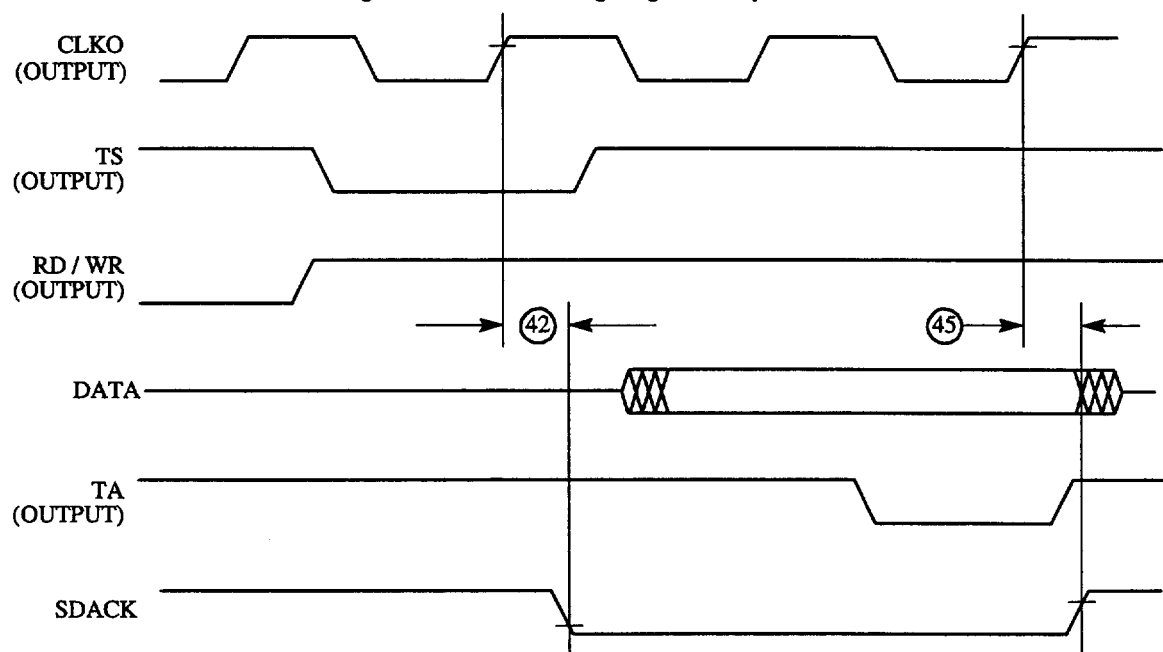
Figure 51 : SDACK Timing Diagram—Peripheral Read
