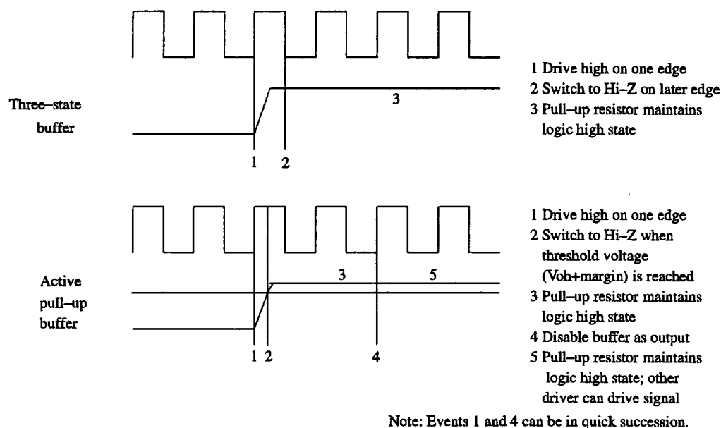
Figure 6 : Three-State Buffers and Active Pull-Up Buffers
