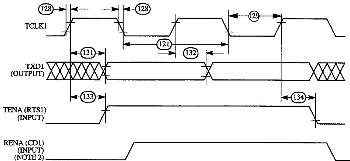
Figure 61 : Ethernet Transmit Timing Diagram
