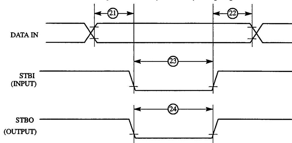
Figure 45 : PIP RX (Pulse Mode) Timing Diagram
