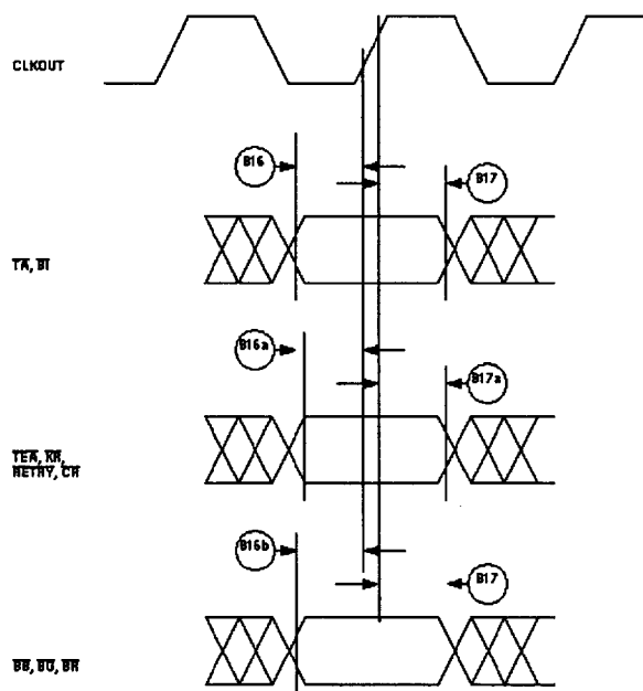
Figure 11 : Synchronous Input Signals Timing
