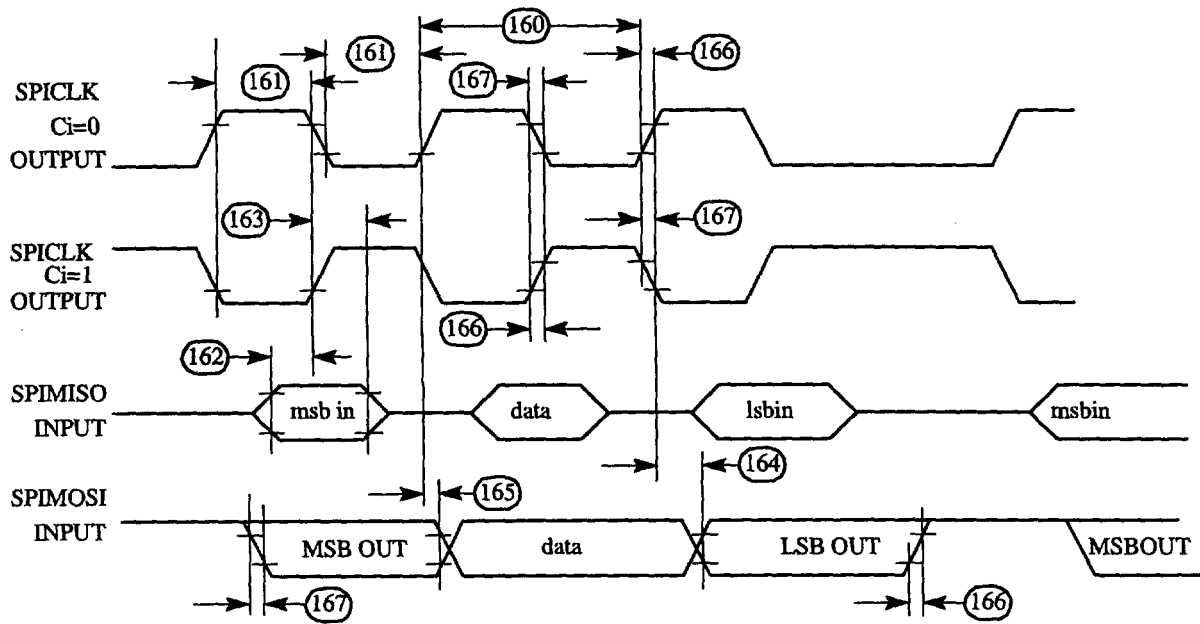
Figure 66 : SPI Master (CP=1) Timing Diagram
