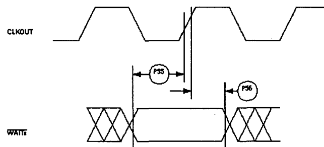
Figure 31 : PCMCIA Wait signals detection Timing
