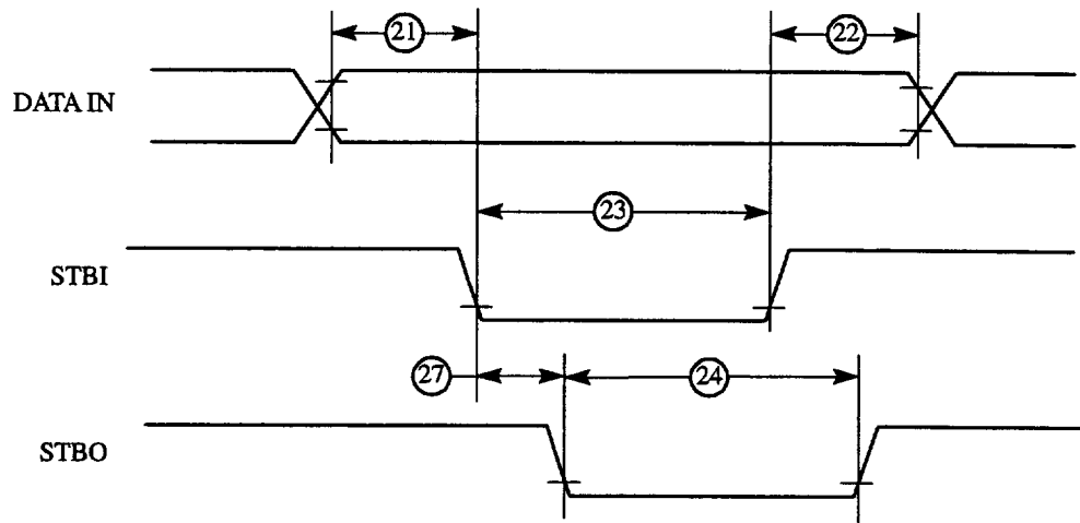
Figure 43 : PIP RX (Interlock Mode) Timing Diagram
