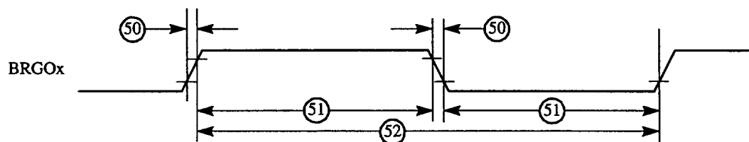
Figure 52 : Baud Rate Generator Timing Diagram
