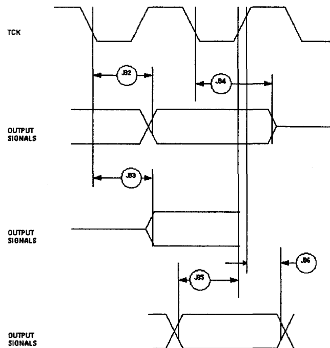
Figure 42 : Boundary Scan (JTAG) Timing Diagram
