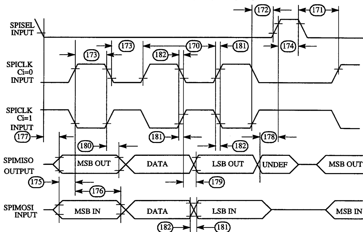
Figure 67 : SPI Slave (CP=0) Timing Diagram
