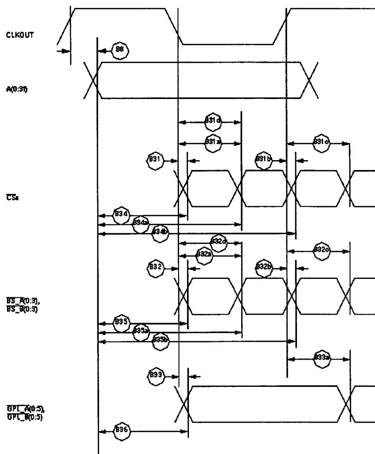
Figure 21 : External Bus Timing (UPM Controlled Signals)
