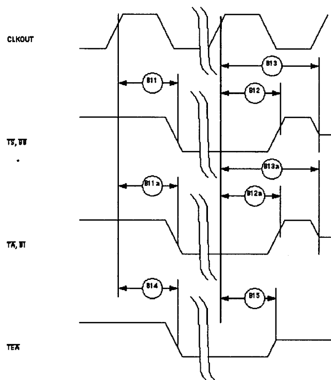
Figure 10 : Synchronous Active Pullup And Open Drain Outputs Signals Timing
