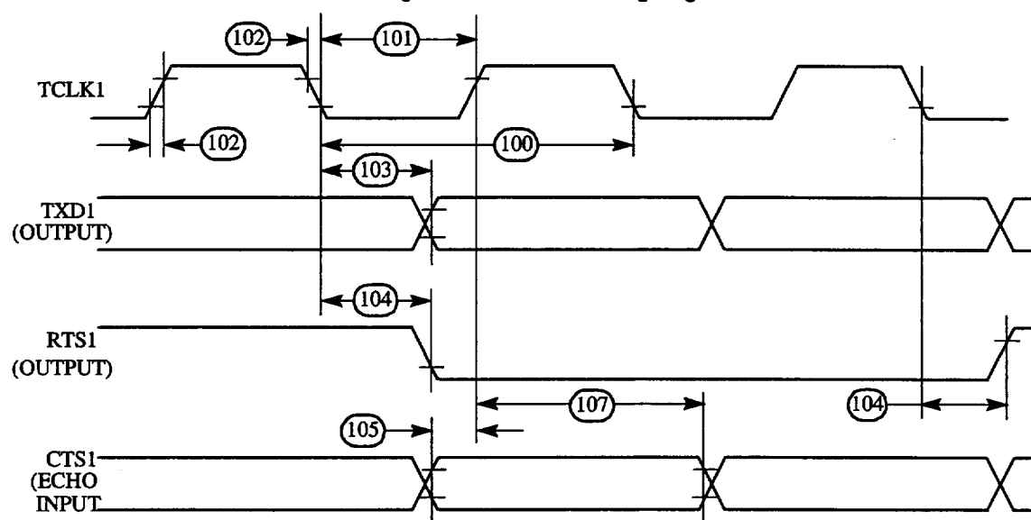
Figure 58 : HDLC Bus Timing Diagram
