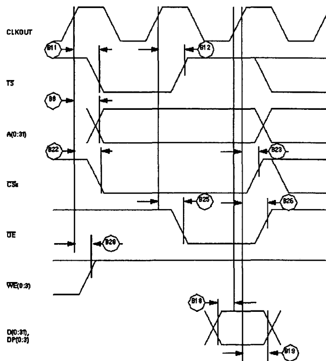
Figure 14 : External Bus Read Timing (GPCM Controlled – ACS = '00')
