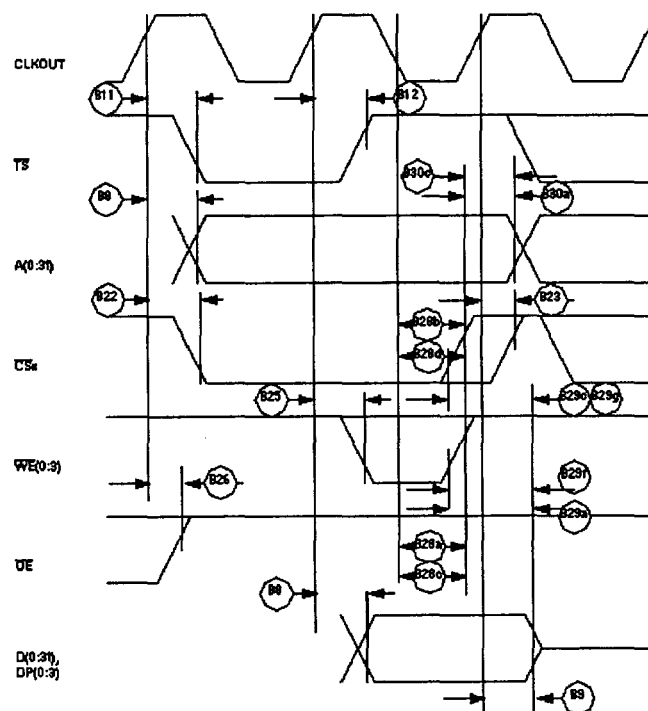
Figure 19 : External Bus Write Timing (GPCM controlled – TRLX = '0', CSNT = '1')
