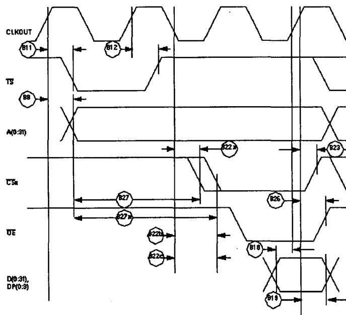
Figure 17 : External Bus Read Timing (GPCM Controlled – TRLX = '1', ACS = '10', ACS = '11')
