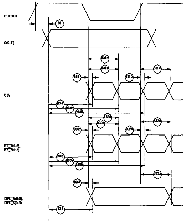
Figure 22 : Asynchronous UPWAIT asserted detection in UPM handled cycles Timing
