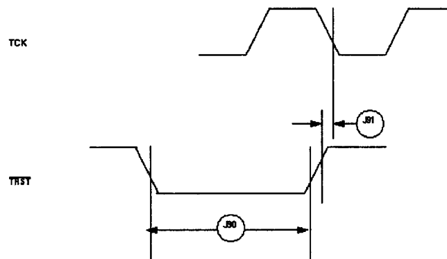
Figure 41 : JTAG—TRST Timing Diagram
