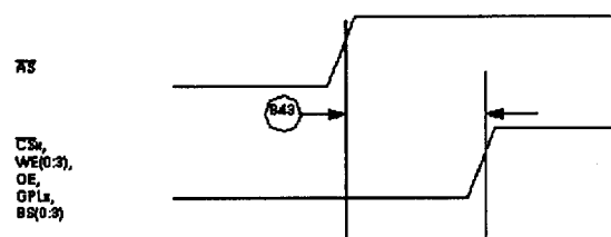
Figure 26 : Asynchronous External Master – Control Signals Negation Time
