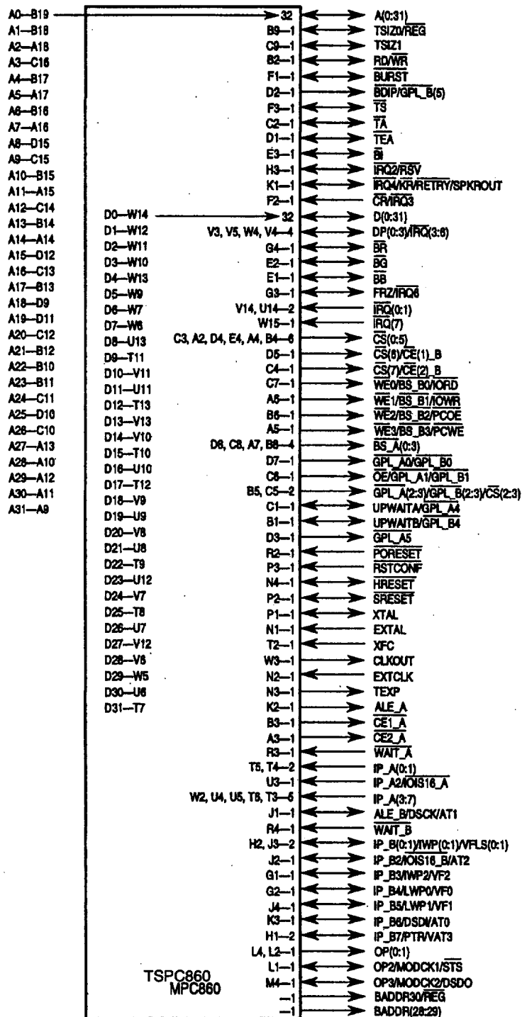
Figure 5 : TSPC860 Signals and Pin Numbers (Part 2)
