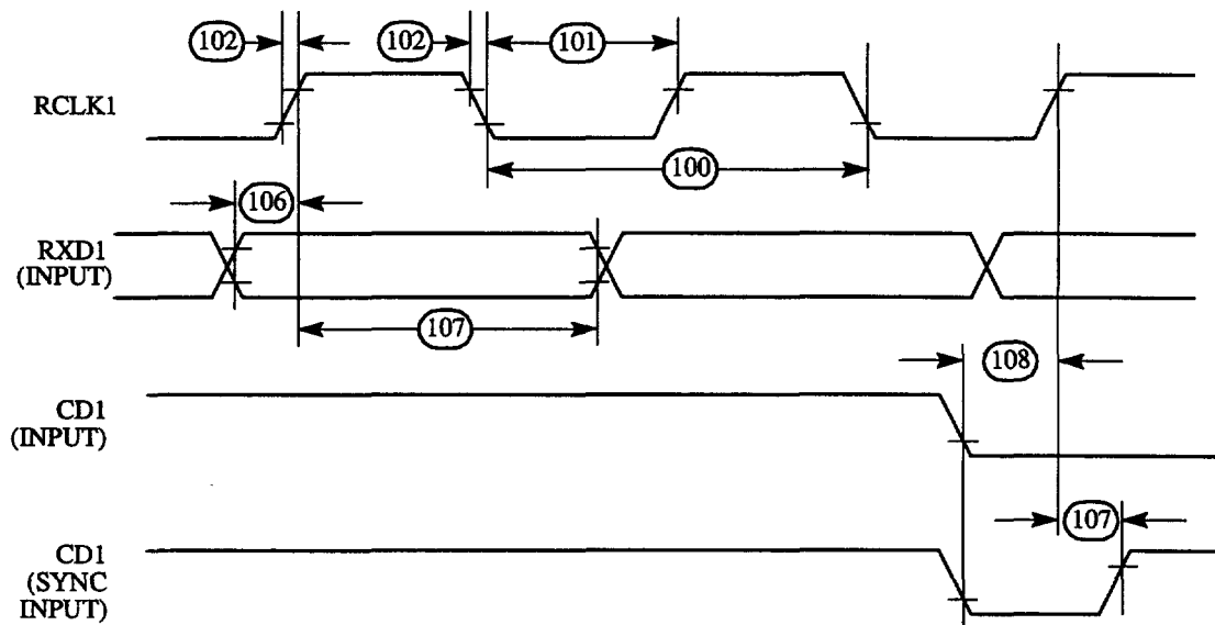
Figure 56 : SCC NMSI Receive Timing Diagram
