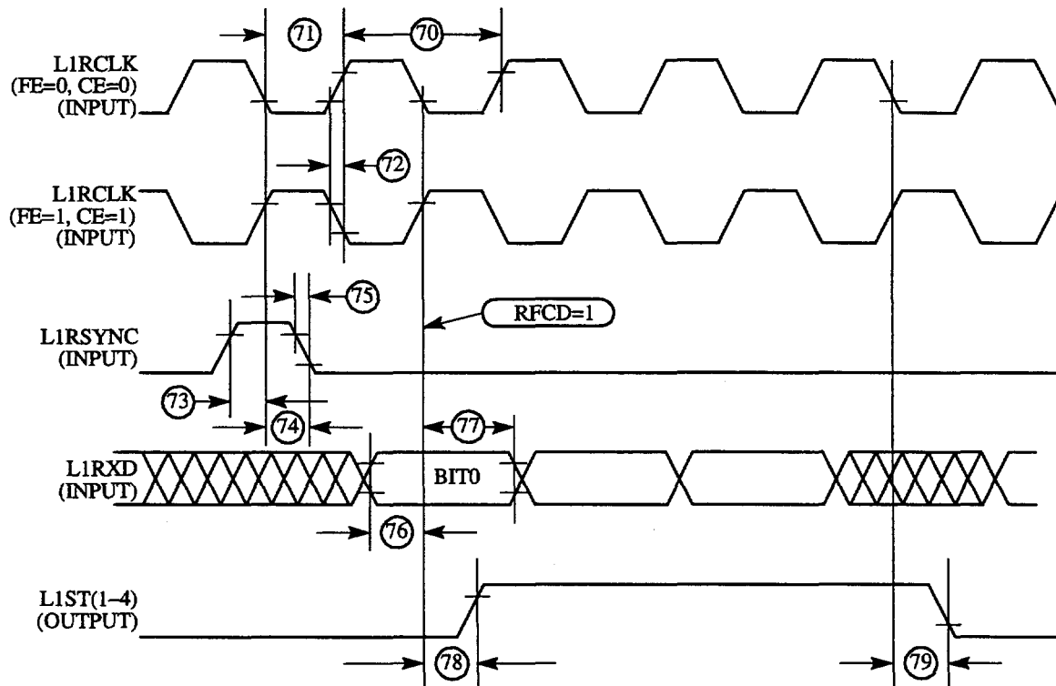
Figure 54 : SI Receive Timing Diagram With Normal Clocking (DSC =0)
