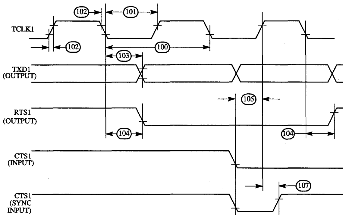
Figure 57 : SCC NMSI Transmit Timing Diagram
