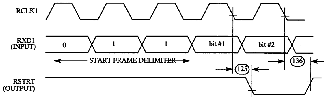
Figure 62 : CAM Interface Receive Start Timing Diagram
