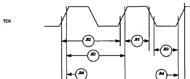
Figure 39 : JTAG Test Clock Input Timing
