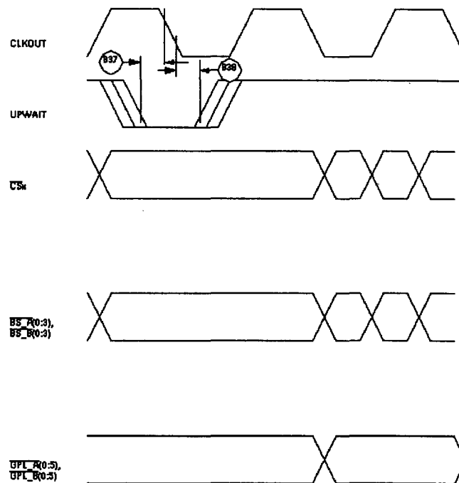
Figure 23 : Asynchronous UPWAIT negated detection in UPM handled cycles Timing
