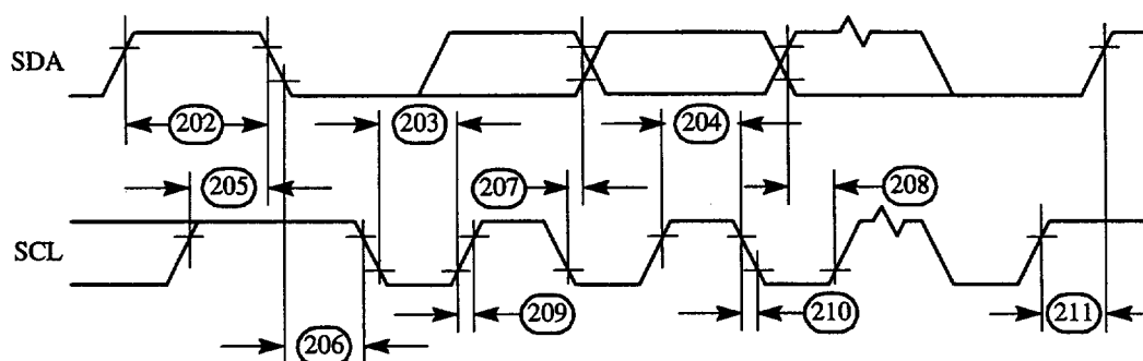
Figure 69 : I 2 C Bus Timing Diagram
