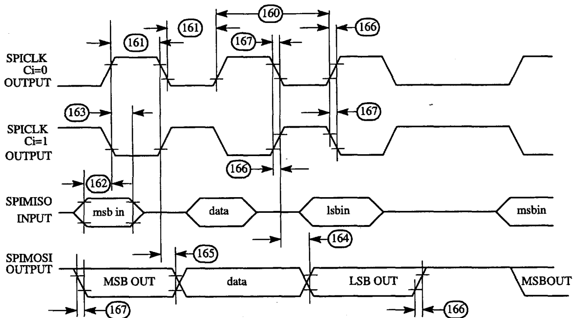
Figure 65 : SPI Master (CP=0) Timing Diagram
