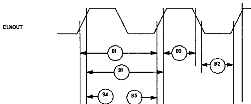
Figure 8 : External Clock Timing
