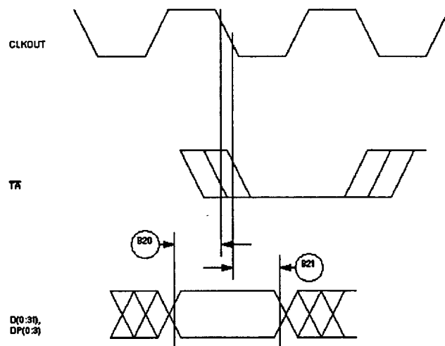
Figure 13 : Input Data Timing when controlled by UPM in the Memory Controller
