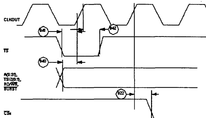
Figure 24 : Synchronous External Master Access Timing – GPCM handled ACS = '00'
