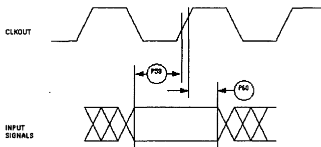
Figure 33 : PCMCIA Input Port Timing
