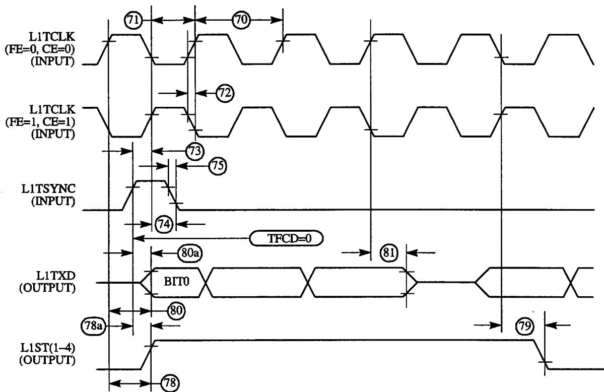
Figure 55 : SI Transmit Timing Diagram
