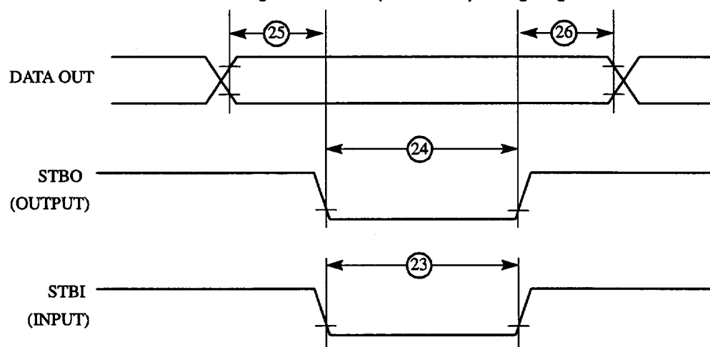
Figure 46 : PIP TX (Pulse Mode) Timing Diagram
