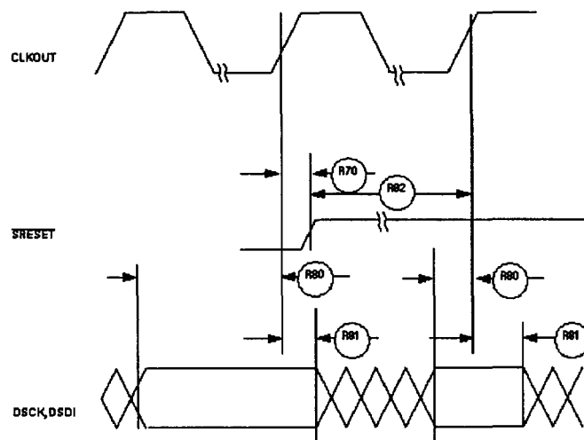
Figure 38 : Reset Timing – Debug Port Configuration
