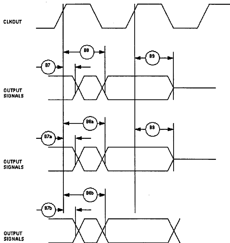
Figure 9 : Synchronous Output Signals Timing
