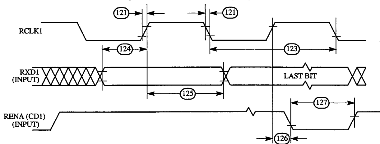
Figure 60 : Ethernet Receive Timing Diagram
