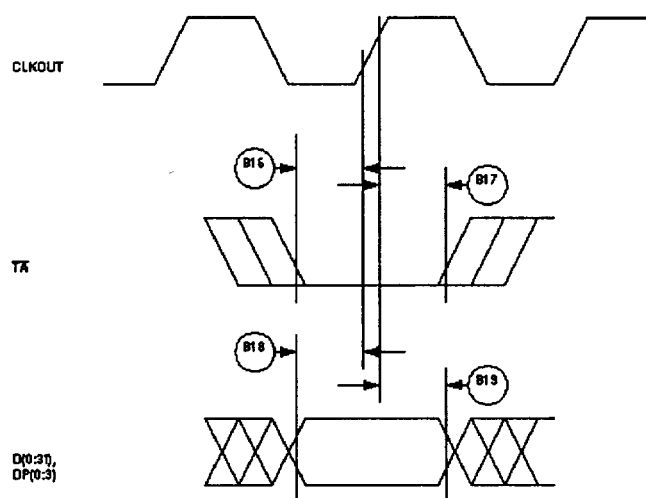
Figure 12 : Input Data Timing In Normal case
