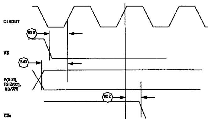
Figure 25 : Asynchronous External Master Memory Access Timing (GPCM Controlled—ACS = '00')
