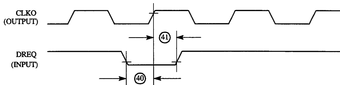
Figure 48 : IDMA External Requests Timing Diagram
