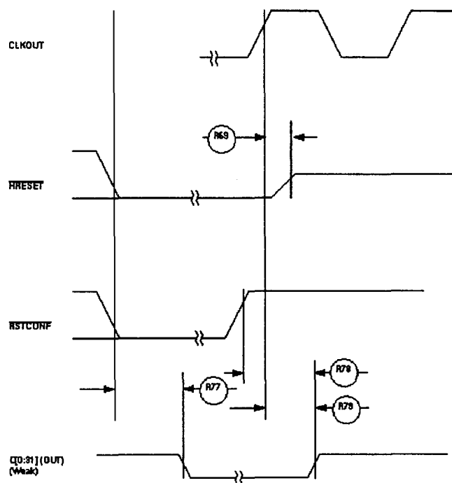
Figure 37 : Reset Timing – TSPC860 Data bus weak drive during Configuration
