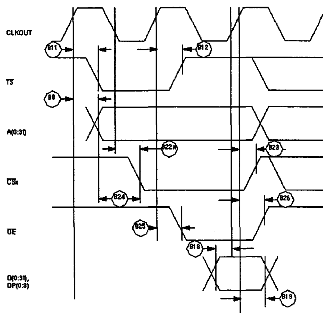
Figure 15 : External Bus Read Timing (GPCM Controlled – TRLX = '0' ACS = '10')
