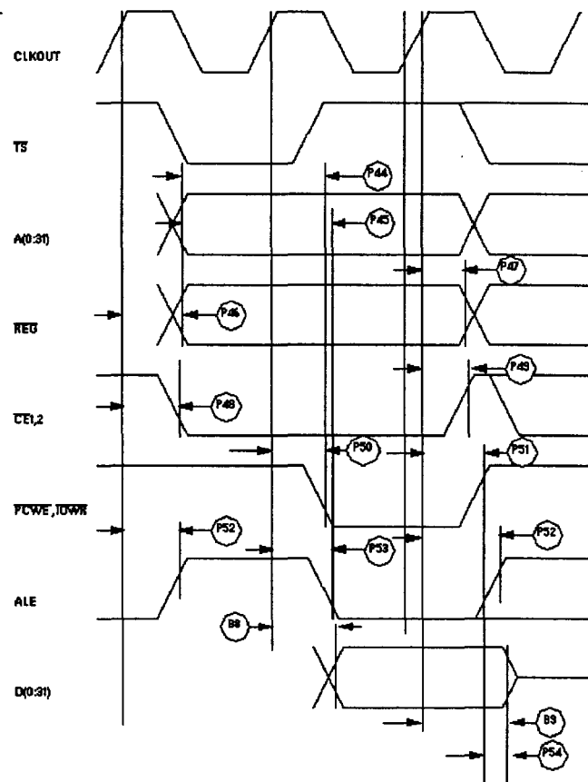
Figure 30 : PCMCIA access cycles Timing External Bus Write
