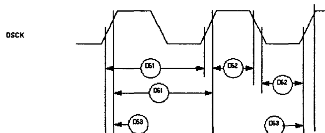
Figure 34 : Debug Port Clock Input Timing
