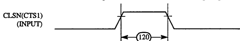
Figure 59 : Ethernet Collision Timing Diagram
