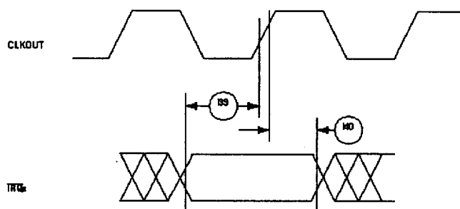
Figure 27 : Interrupt Detection Timing for External Level Sensitive Lines
