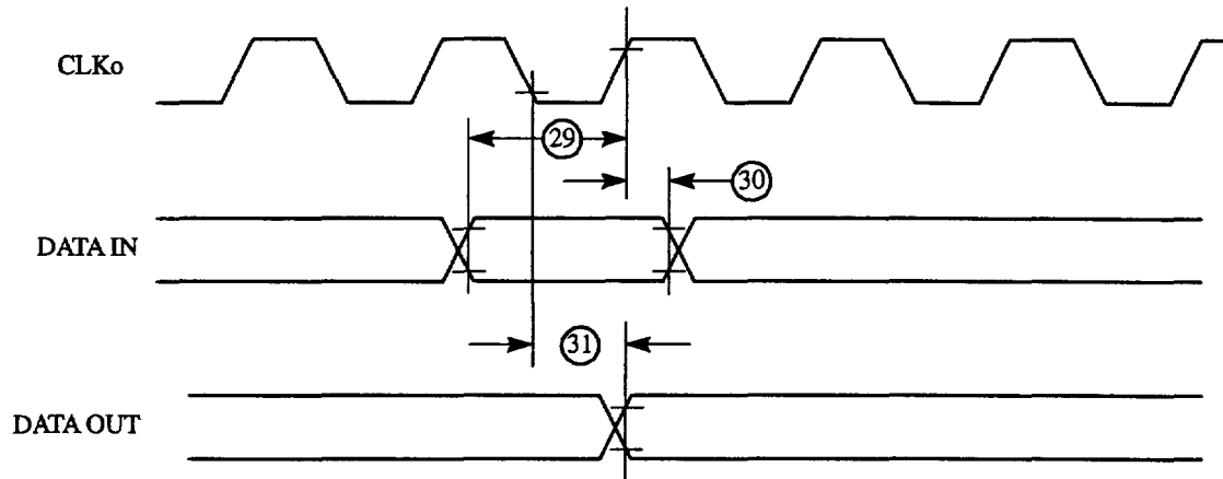
Figure 47 : Parallel I/O Data-In/Data-Out Timing Diagram
