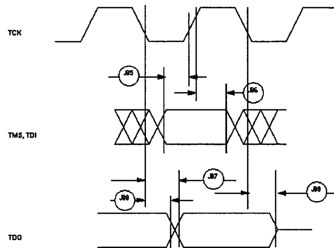
Figure 40 : JTAG—Test Access Port Timing Diagram
