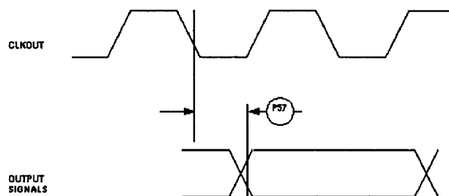
Figure 32 : PCMCIA Output port timing
