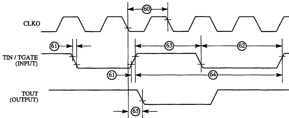
Figure 53 : CPM General-Purpose Timers Timing Diagram
