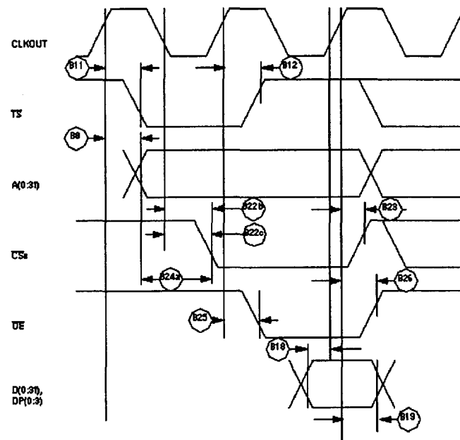
Figure 16 : External Bus Read Timing (GPCM Controlled – TRLX = '0' ACS = '11')
