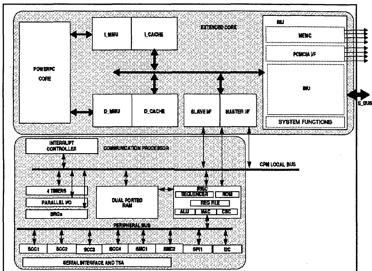
Figure 1 : Block diagram view of the TSPC860
