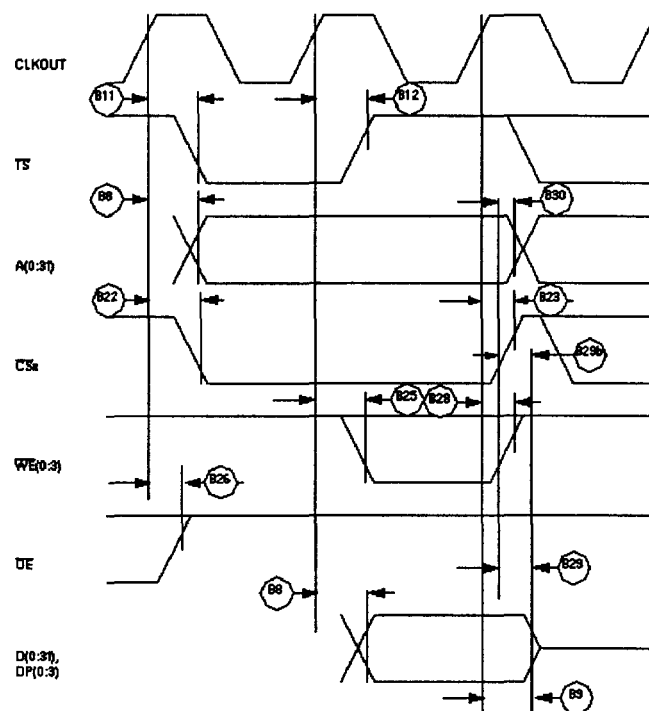
Figure 18 : External Bus Write Timing (GPCM controlled – TR LX = '0', CSNT = '0')
