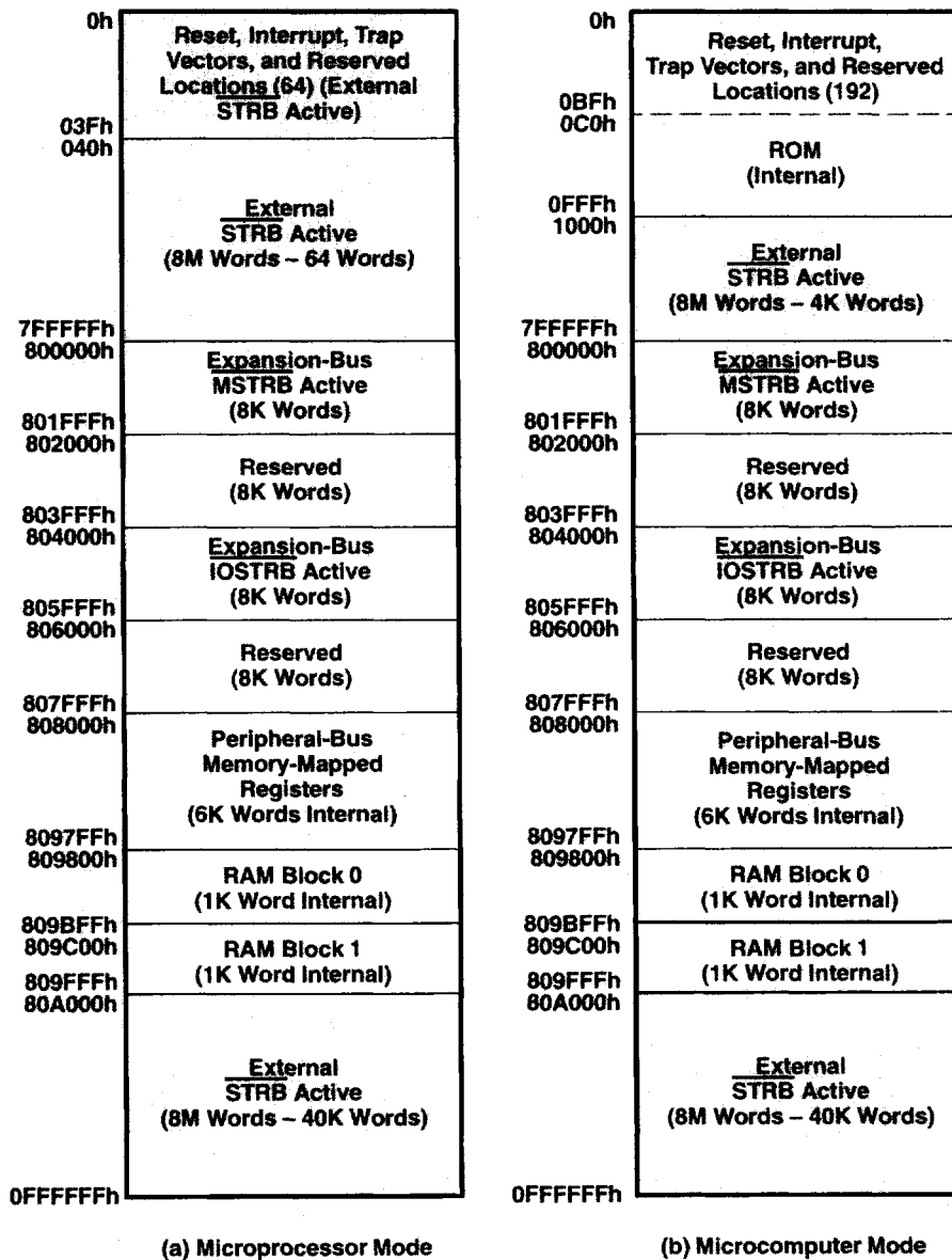
Figure 1. Memory Map
