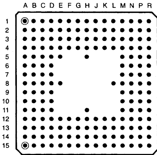
181-Pin GB Grid Array Package (BOTTOM VIEW)
