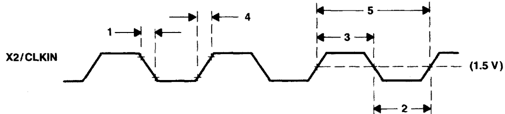
Figure 7. X2/CLKIN Timing
