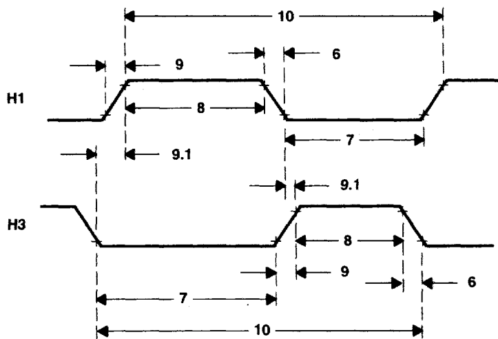
Figure 8. H1/H3 Timings
