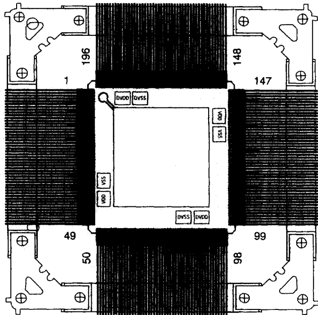
196-Pin HFG Quad Flatpack (TOP VIEW)
