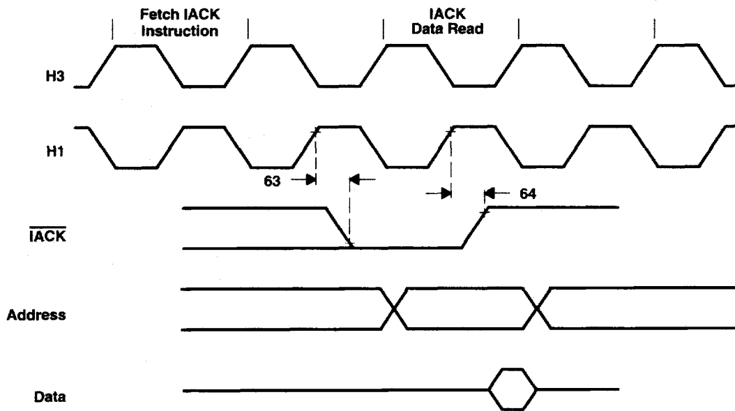
Figure 22. Timing for Interrupt-Acknowledge ( \overline{\text{IACK}} )
