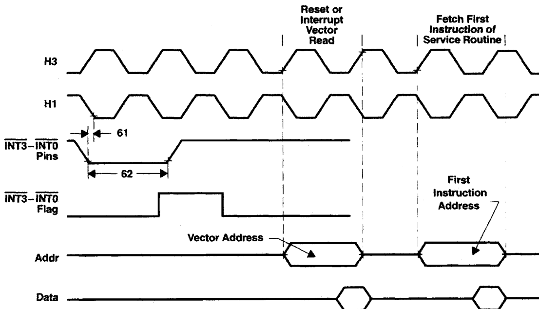
Figure 21. Timing for \overline{\text{INT3}}-\overline{\text{INT0}} Response [ Q = t_{c(H)} ]
