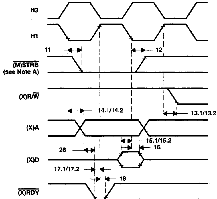
Figure 10. Timing for Memory [(M)STRB = 0] Read
