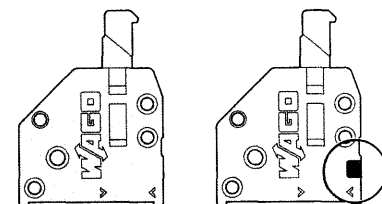
A groove at the back of the terminal block differentiates between the two pin spacings
