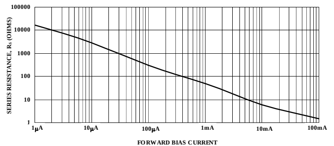
Resistance vs Forward Current (MA4P278 / MA4P7438 /MADP-007438 Series)
