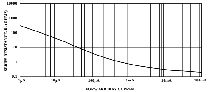
Resistance vs Forward Current (MA4P275 / MA4P7436 /MADP-007436 Series)
