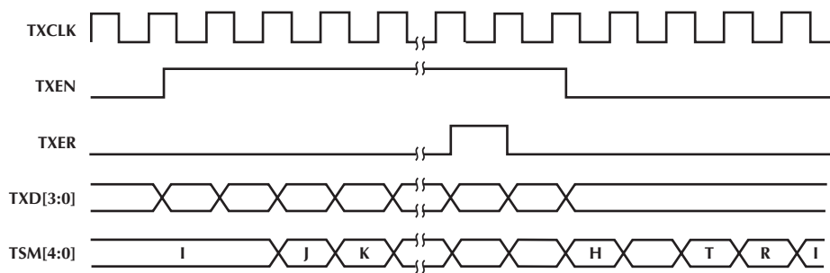
Transmission Timing
