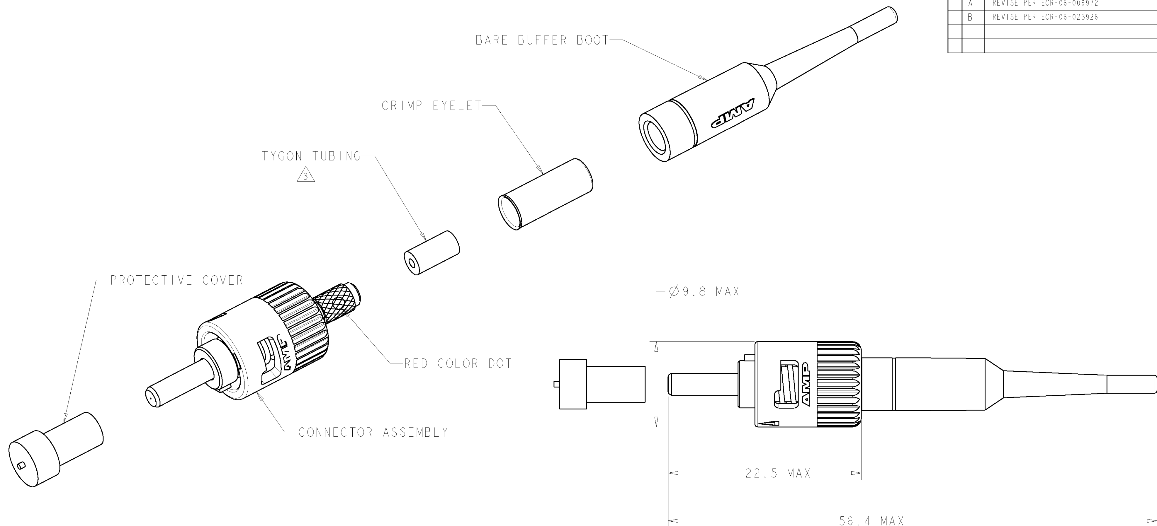
ASSEMBLED CONNECTOR
