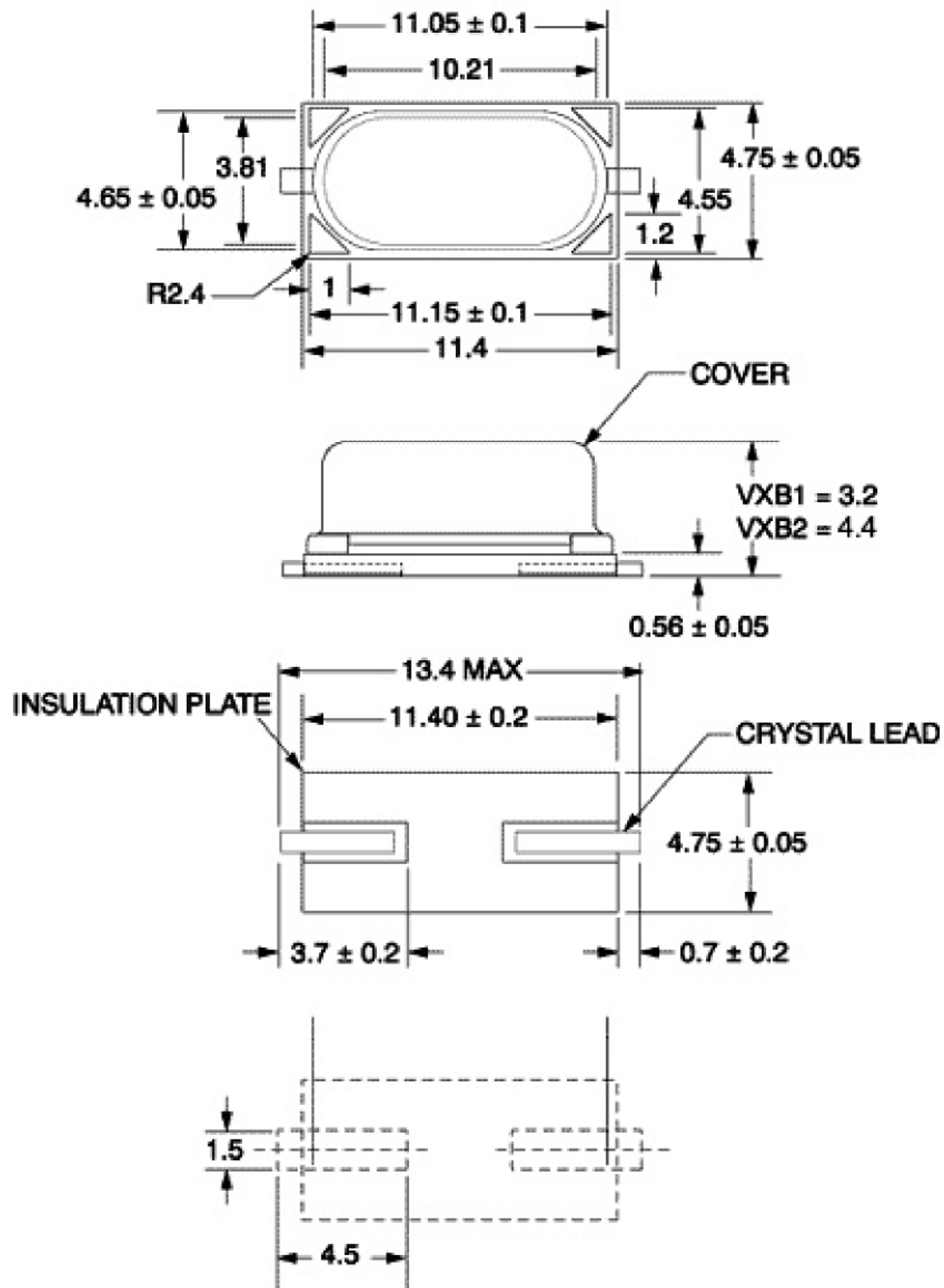
Recommended soldering pattern
