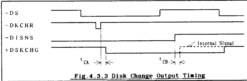
Fig.4.3.3 Disk Change Output Timing
