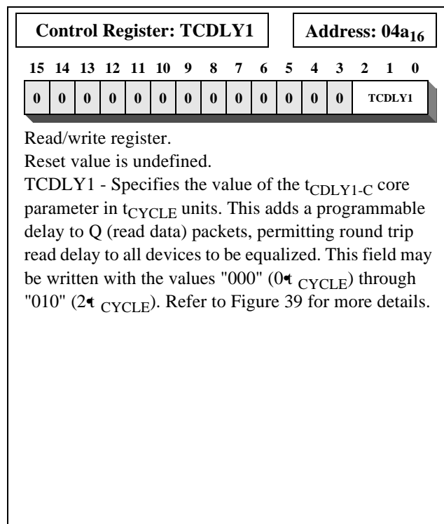
Figure 41: TCDLY Register
