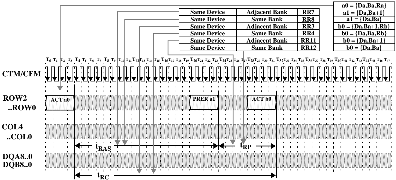
Figure 10: Row Packet Examples
