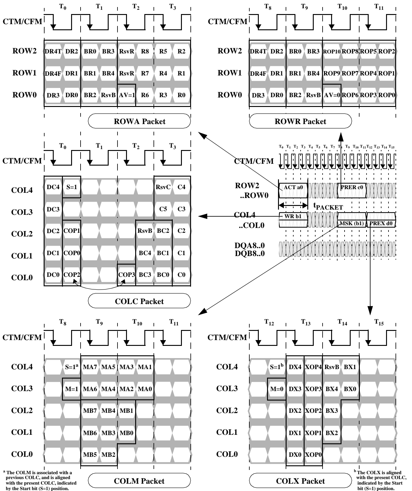
Figure 3: Packet Formats
