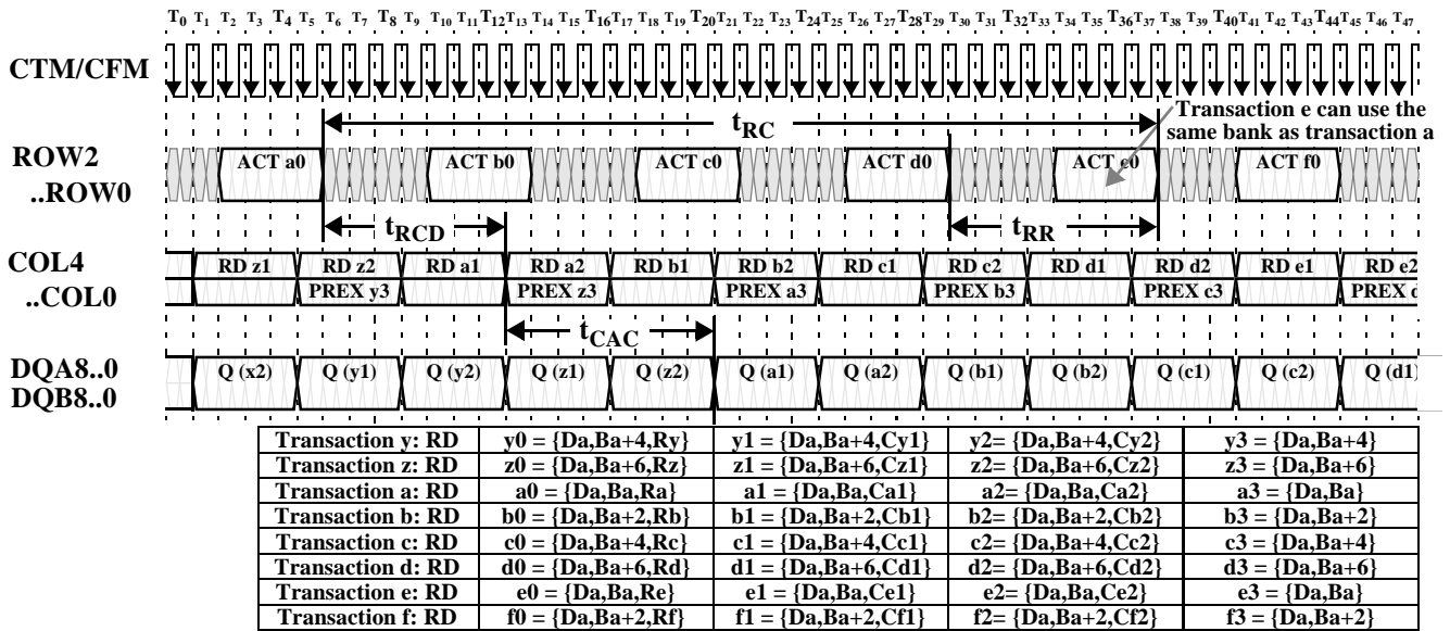
Figure 21: Interleaved Read Transactions with Two Dualoct Data Length
