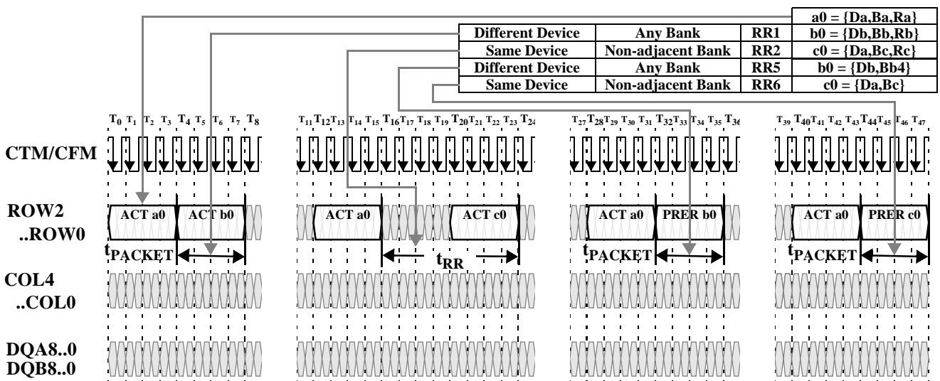
Figure 11: Row Packet Examples
