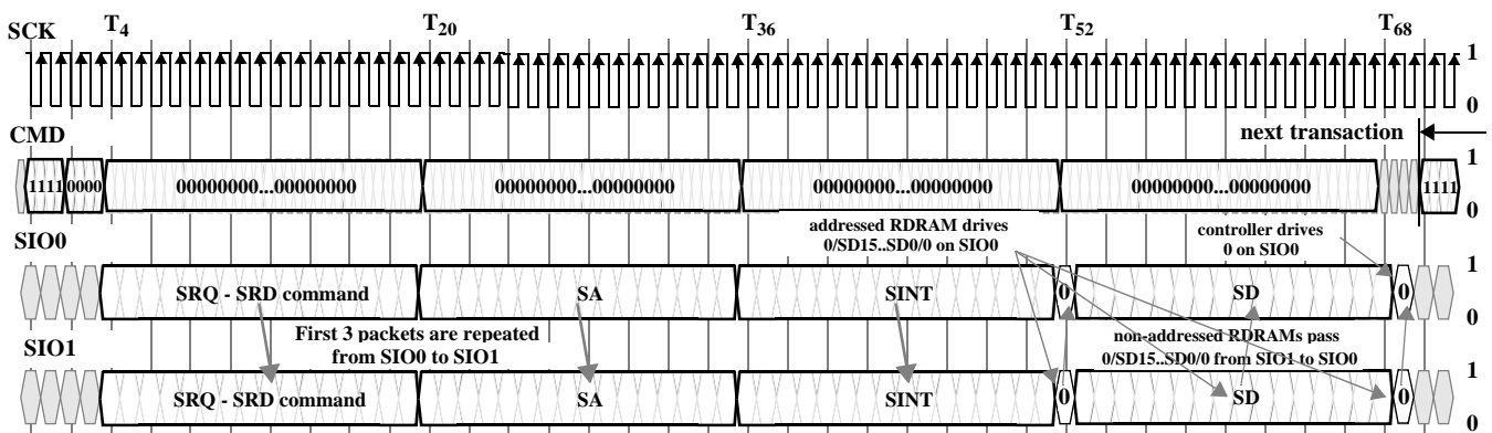
Figure 24: Serial Read (SRD) Transaction to Control Register
