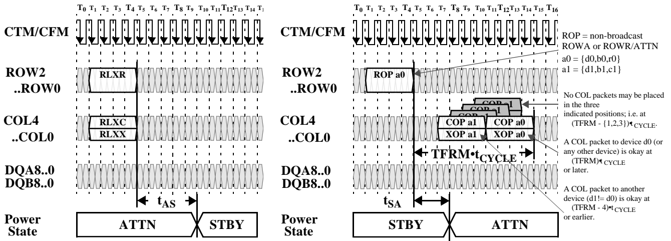
Figure 46: STBY Entry (left) and STBY Exit (right)
